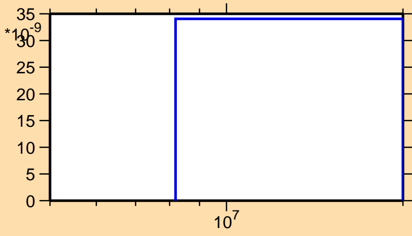
\sigma vs. E for ^{208}\text{Tl}(n,nt)
