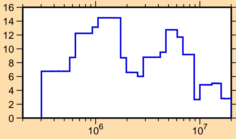
\Delta\sigma/\sigma vs. E for ^{209}\text{Tl}(n,\text{el.})
