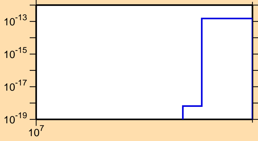
\sigma vs. E for ^{209}\text{Tl} (mt 42)
