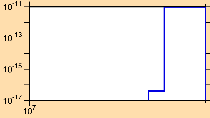
\sigma vs. E for ^{209}\text{Tl} (mt 11)
