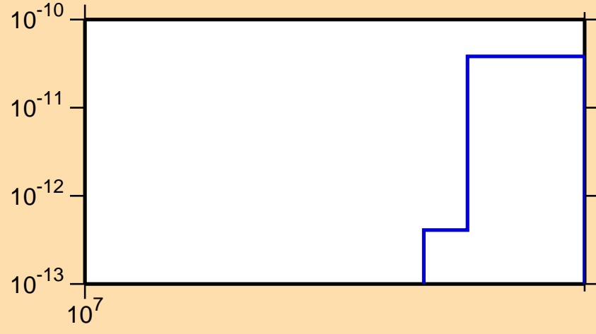
\sigma vs. E for ^{209}\text{Tl}(n,3n\alpha)
