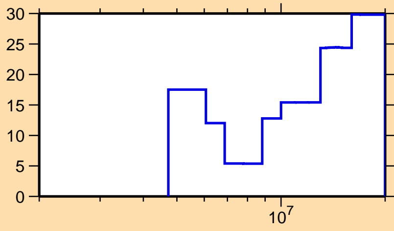
\Delta\sigma/\sigma vs. E for ^{209}\text{Tl}(n,2n)
