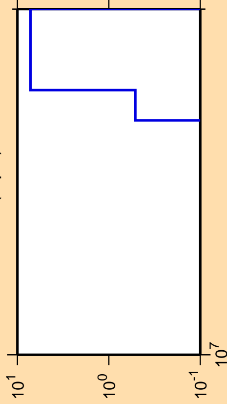
\Delta\sigma/\sigma vs. E for ^{209}\text{Tl}(n,p\alpha)
