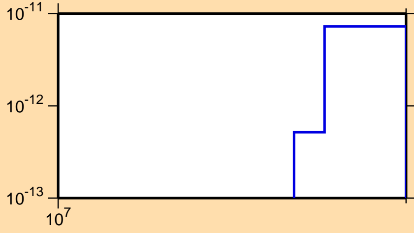
\sigma vs. E for ^{209}\text{Tl}(n,p\alpha)
