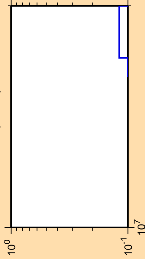
\Delta\sigma/\sigma vs. E for ^{209}\text{Tl} (mt 42)
