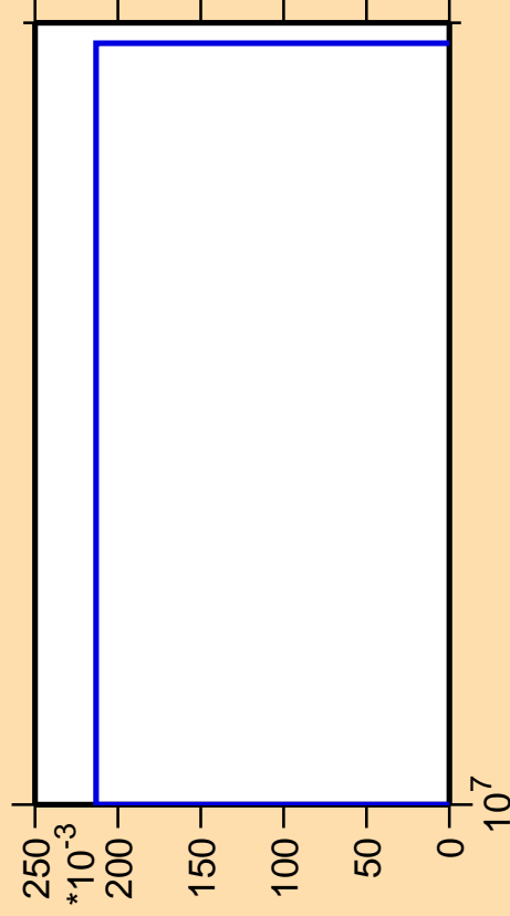
\Delta\sigma/\sigma vs. E for ^{209}\text{Tl} (mt 11)
