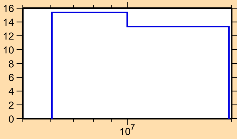
\Delta\sigma/\sigma vs. E for ^{209}\text{Tl}(n,n_1)
