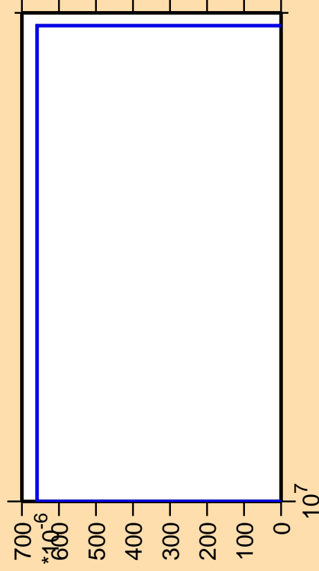
\Delta\sigma/\sigma vs. E for ^{209}\text{Tl} (mt 42)
