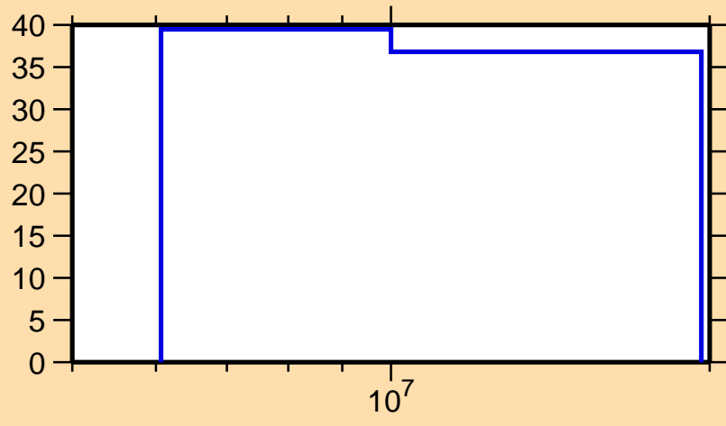
\Delta\sigma/\sigma vs. E for ^{209}\text{Tl}(n,p)
