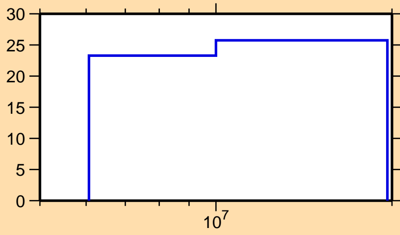
\Delta\sigma/\sigma vs. E for ^{209}\text{Tl}(n,ncont.)
