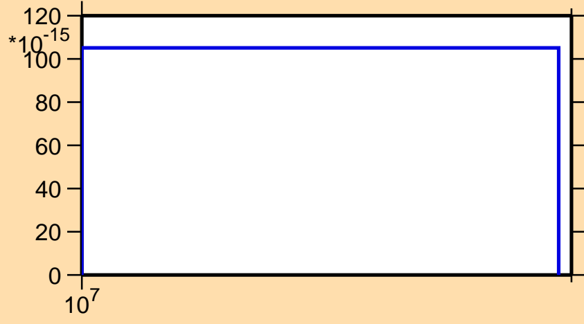
\sigma vs. E for ^{209}\text{Tl}(n,p\alpha)
