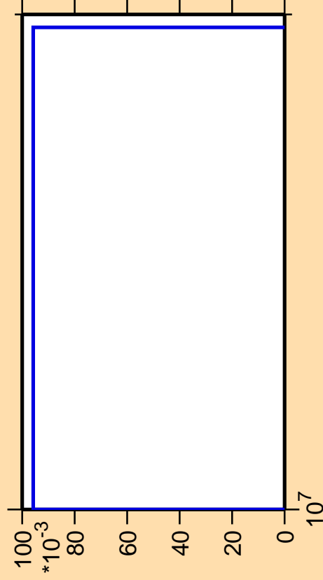
\Delta\sigma/\sigma vs. E for ^{209}\text{Tl}(n,p\alpha)
