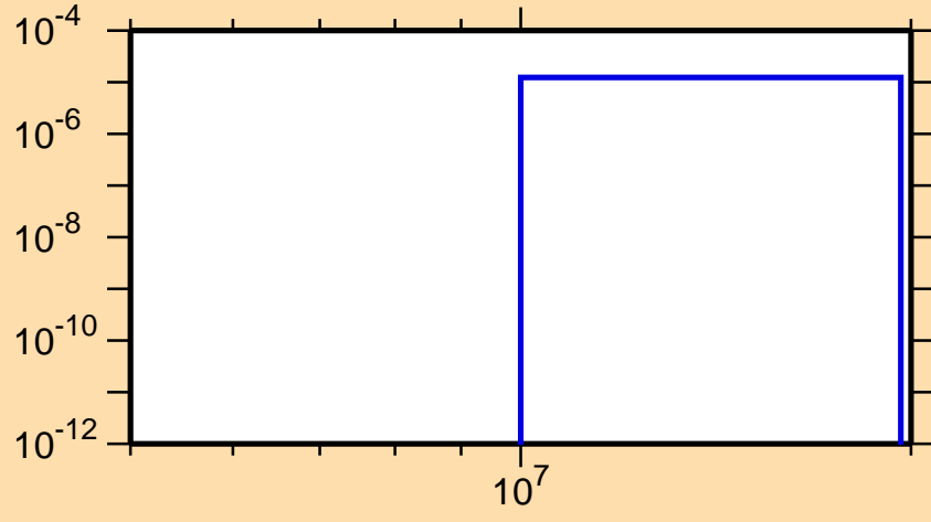
\sigma vs. E for ^{209}\text{Tl}(n,np)
