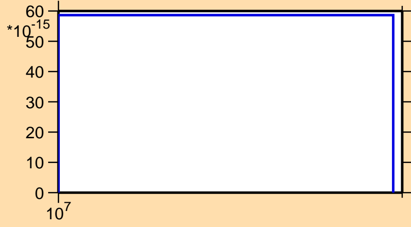
\sigma vs. E for ^{209}\text{Tl} (mt 11)
