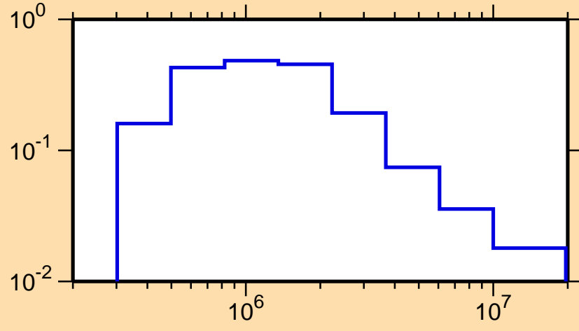
\sigma vs. E for ^{209}\text{Tl}(n,n_1)
