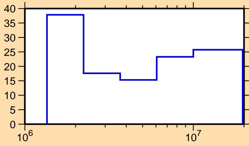
\Delta\sigma/\sigma vs. E for ^{209}\text{Tl}(n,n\text{cont.})
