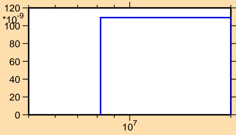
\sigma vs. E for ^{210}\text{Tl}(n,nd)
