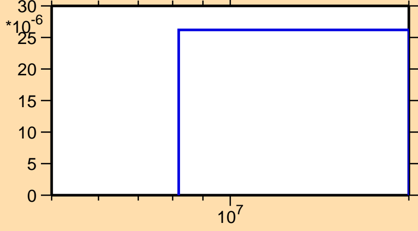
\sigma vs. E for ^{210}\text{Tl}(n,d)
