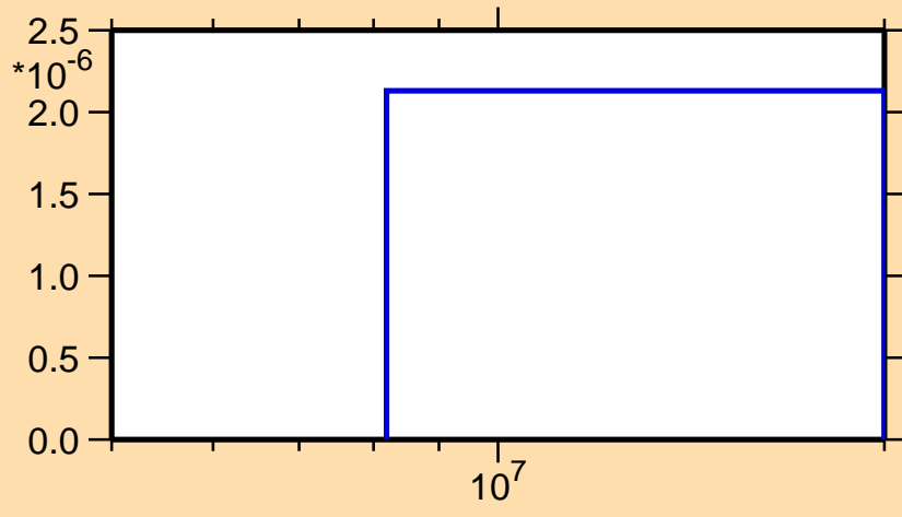
\sigma vs. E for ^{210}\text{Tl}(n,nt)
