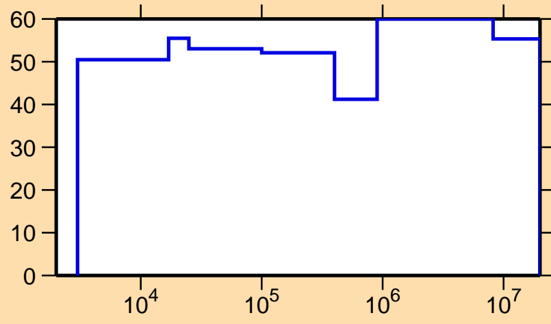
\Delta\sigma/\sigma vs. E for ^{210}\text{Tl}(n,\gamma)
