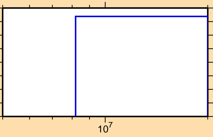
\sigma vs. E for ^{210}\text{Tl}(n,np)
