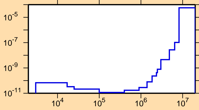
\sigma vs. E for ^{210}\text{Tl}(n,\alpha)
