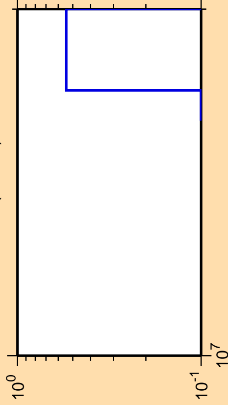
\Delta\sigma/\sigma vs. E for ^{211}\text{Tl} (mt 42)
