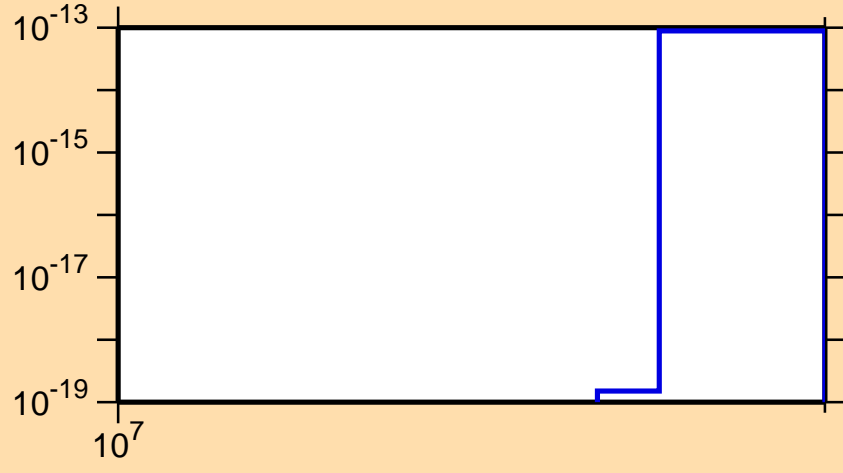
\sigma vs. E for ^{211}\text{Tl} (mt 42)
