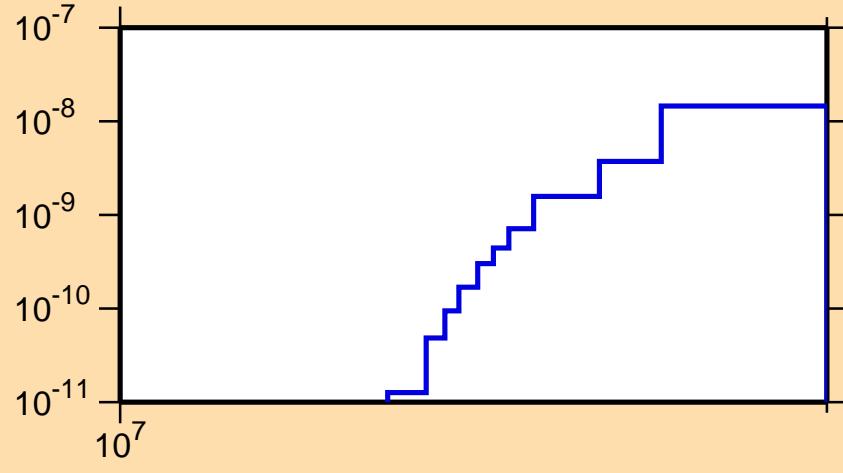
\sigma vs. E for ^{211}\text{Tl}(n,3n\alpha)
