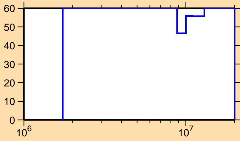
\Delta\sigma/\sigma vs. E for ^{211}\text{Tl}(n,\gamma)
