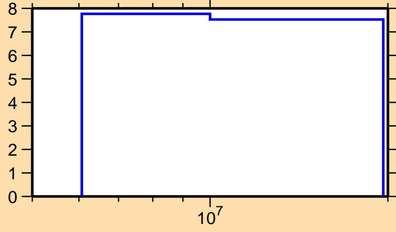
\Delta\sigma/\sigma vs. E for ^{212}\text{Tl}(n,\text{nonel.})
