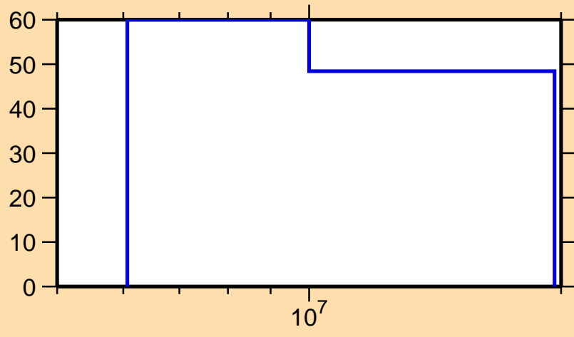
\Delta\sigma/\sigma vs. E for ^{212}\text{Tl}(n,p)
