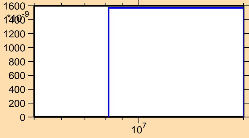
\sigma vs. E for ^{212}\text{Tl}(n,nt)
