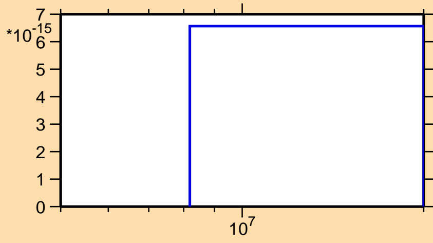
\sigma vs. E for ^{212}\text{Tl} (mt 42)
