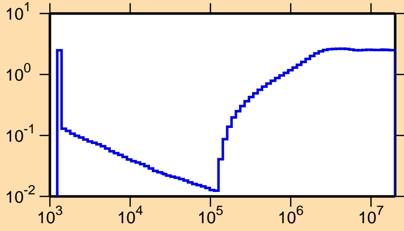
\sigma vs. E for ^{213}\text{Tl}(n,\text{nonel.})
