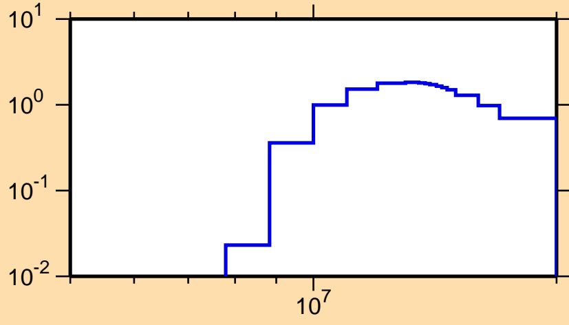
\sigma vs. E for ^{214}\text{Tl}(n,3n)
