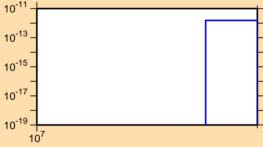
\sigma vs. E for ^{214}\text{Tl} (mt 42)
