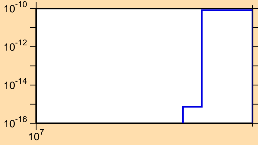
\sigma vs. E for ^{214}\text{Tl} (mt 11)
