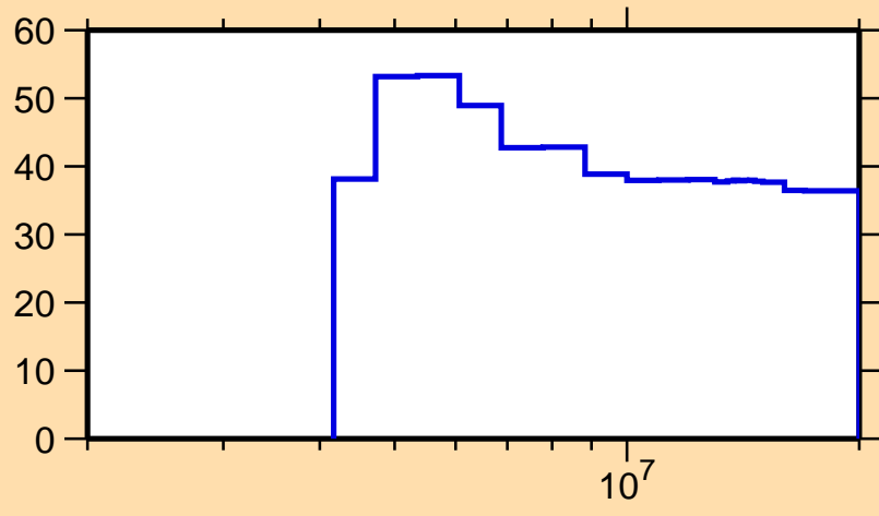
\Delta\sigma/\sigma vs. E for ^{214}\text{Tl}(n,n\text{cont.})
