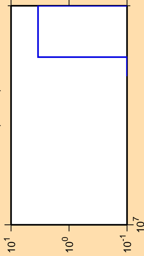
\Delta\sigma/\sigma vs. E for ^{214}\text{Tl} (mt 42)
