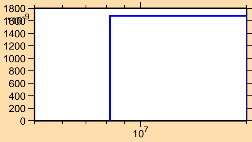
\sigma vs. E for ^{214}\text{Tl}(n,nt)
