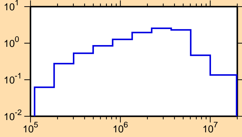
\sigma vs. E for ^{215}\text{Tl}(n,\text{inel.})
