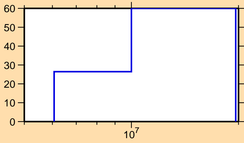
\Delta\sigma/\sigma vs. E for ^{215}\text{Tl}(n,p)
