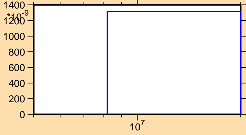
\sigma vs. E for ^{215}\text{Tl}(n,nt)
