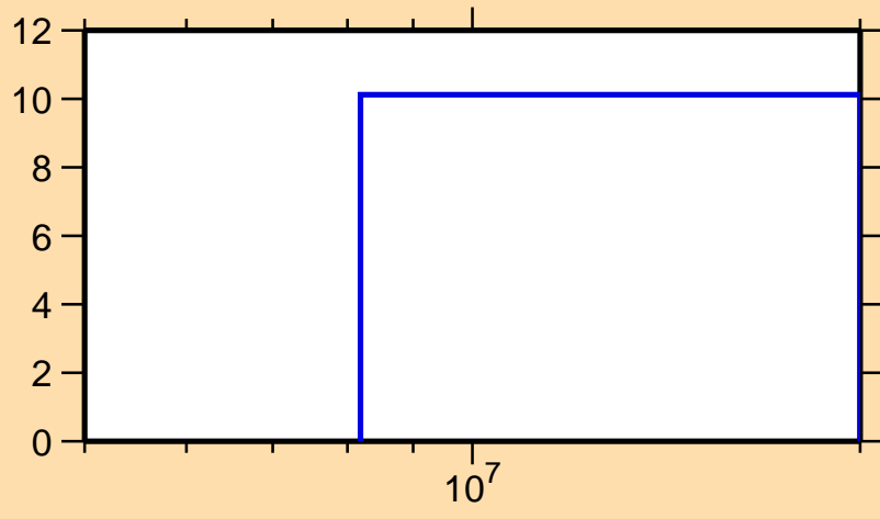
\Delta\sigma/\sigma vs. E for ^{215}\text{Tl}(n,el.)
