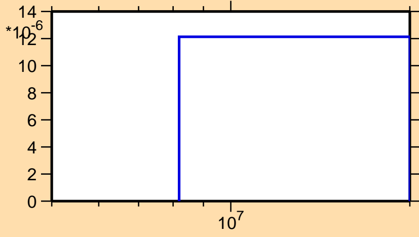
\sigma vs. E for ^{215}\text{Tl}(n,t)
