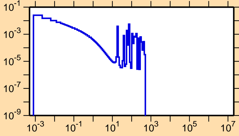
\sigma vs. E for ^{216}\text{Tl}(n,f)
