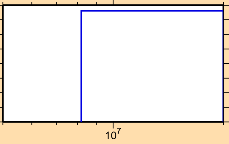
\sigma vs. E for ^{216}\text{Tl}(n,np)
