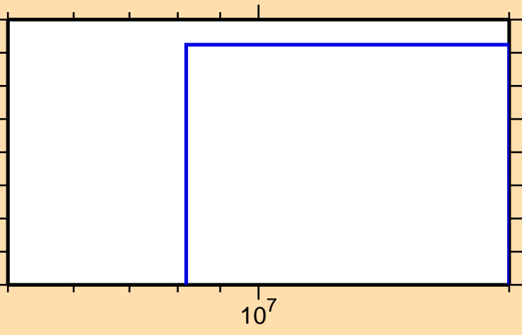
\sigma vs. E for ^{216}\text{Tl}(n,nt)
