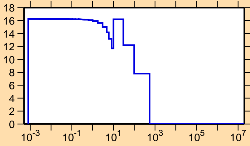
\Delta\sigma/\sigma vs. E for ^{216}\text{Tl}(n,f)
