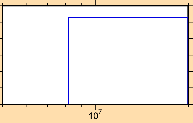
\sigma vs. E for ^{216}\text{Tl}(n,3n\alpha)
