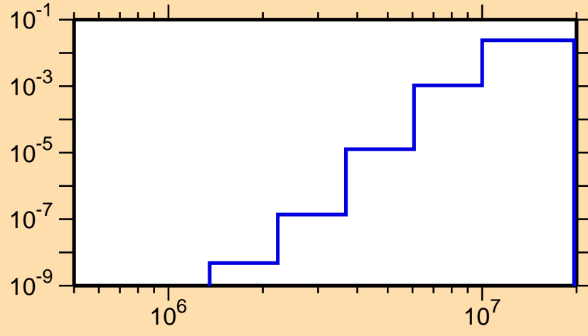
\sigma vs. E for ^{150}\text{Tm}(n,d)
