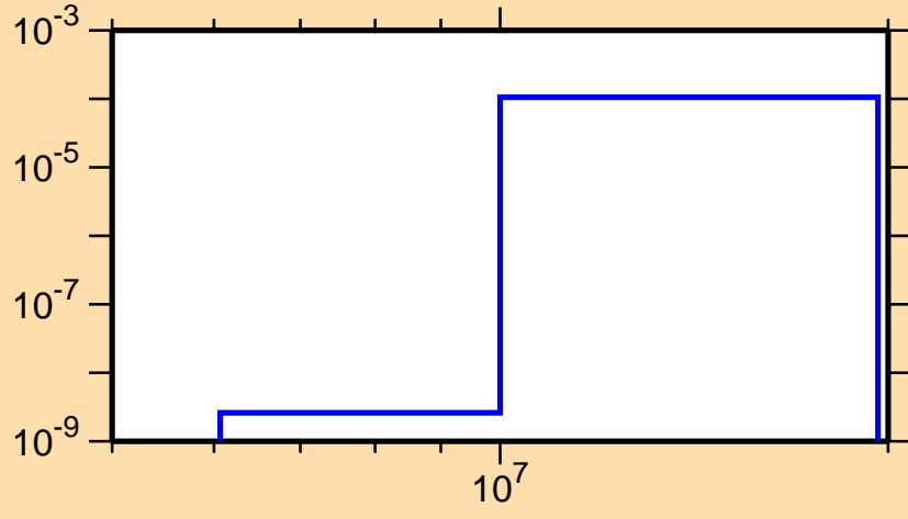
\sigma vs. E for ^{150}\text{Tm} (mt 45)
