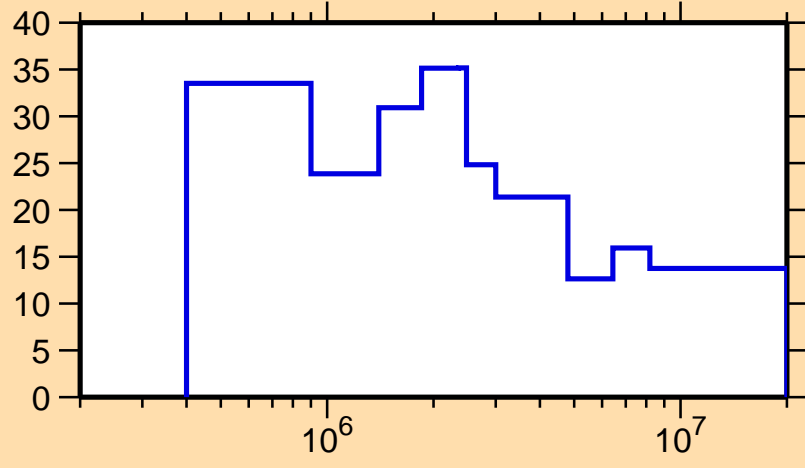
\Delta\sigma/\sigma vs. E for ^{150}\text{Tm}(n, el.)
