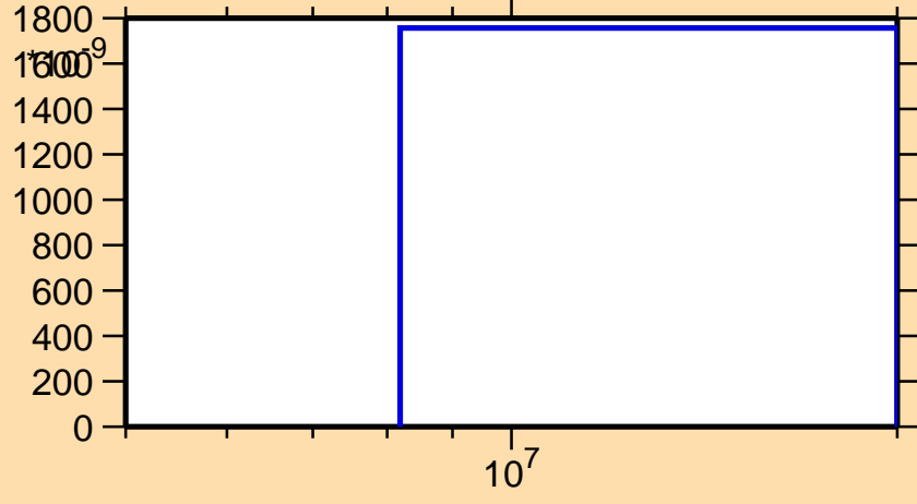
\sigma vs. E for ^{150}\text{Tm}(n,pt)
