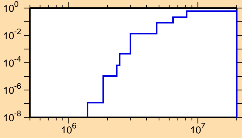
\sigma vs. E for ^{150}\text{Tm}(n,np)
