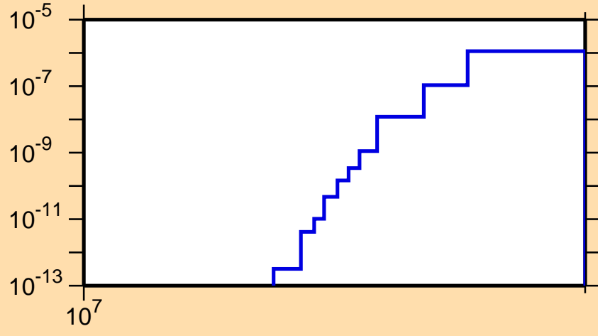
\sigma vs. E for ^{151}\text{Tm}(n,nd)
