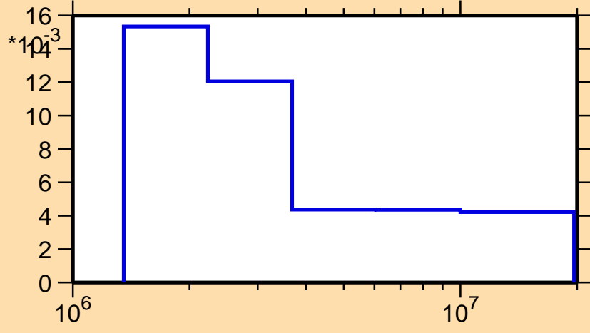
\sigma vs. E for ^{151}\text{Tm}(n,n_3)
