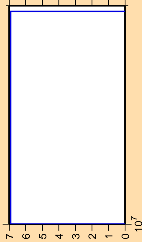
\Delta\sigma/\sigma vs. E for ^{151}\text{Tm} (mt 34)
