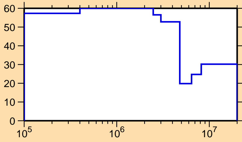
\Delta\sigma/\sigma vs. E for ^{151}\text{Tm}(n,n_1)
