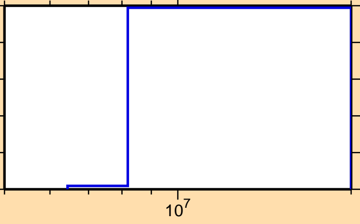
\sigma vs. E for ^{151}\text{Tm}(\text{mt117})
