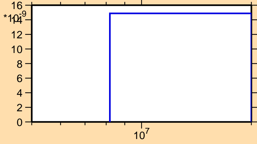
\sigma vs. E for ^{151}\text{Tm}(n,\text{nd})
