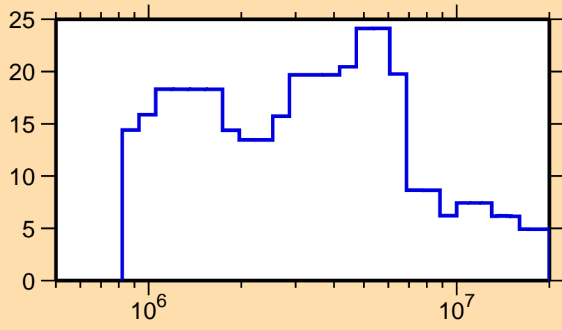
\Delta\sigma/\sigma vs. E for ^{151}\text{Tm}(n, el.)
