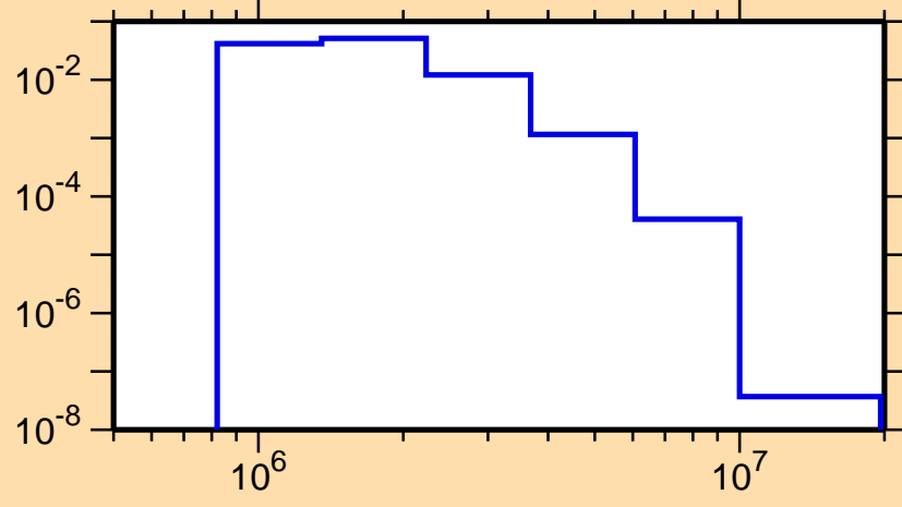
\sigma vs. E for ^{151}\text{Tm}(n,n_2)
