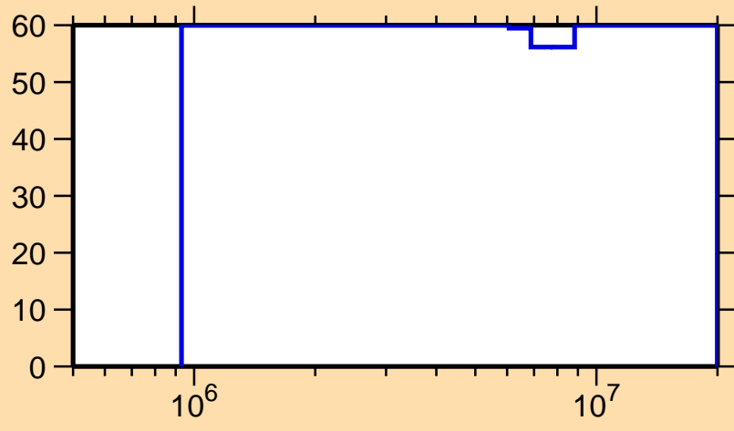
\Delta\sigma/\sigma vs. E for ^{152}\text{Tm}(n,ncont.)
