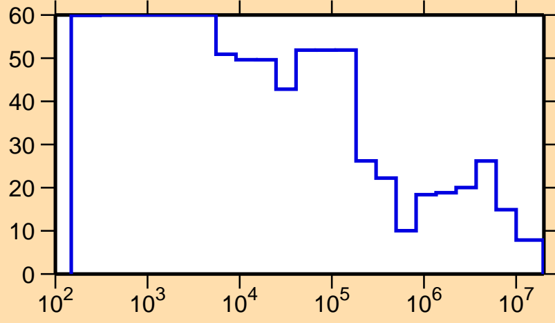
\Delta\sigma/\sigma vs. E for ^{152}\text{Tm}(n,el.)
