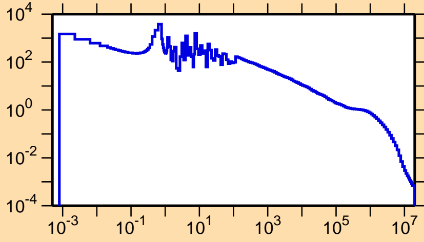
\sigma vs. E for ^{152}\text{Tm}(n,\gamma)
