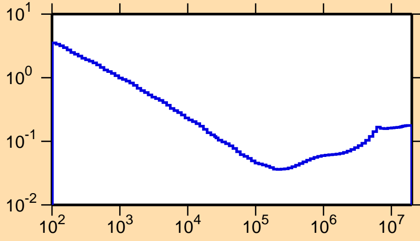
\sigma vs. E for ^{152}\text{Tm}(n,p\alpha)
