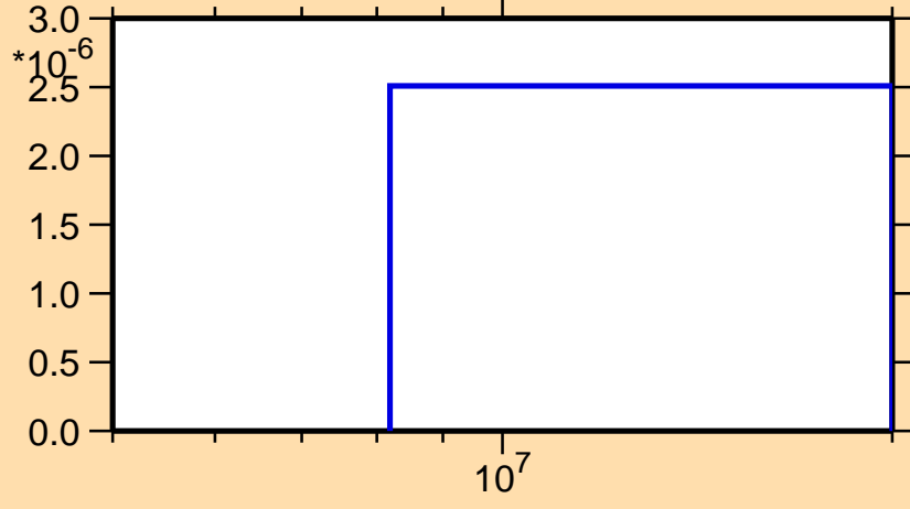
\sigma vs. E for ^{152}\text{Tm}(n,nd)
