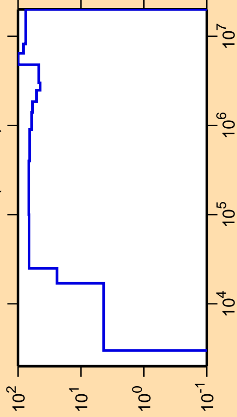
\Delta\sigma/\sigma vs. E for ^{152}\text{Tm}(n,\text{inel.})
