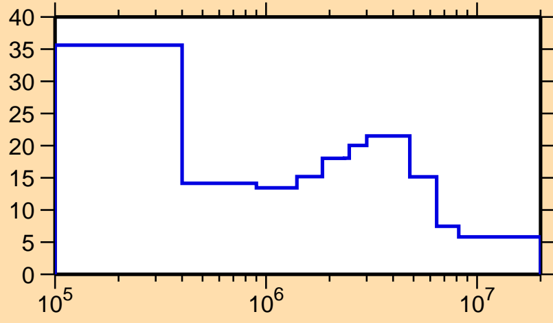
\Delta\sigma/\sigma vs. E for ^{152}\text{Tm}(n, el.)
