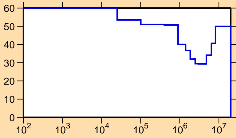
\Delta\sigma/\sigma vs. E for ^{152}\text{Tm}(n,p)
