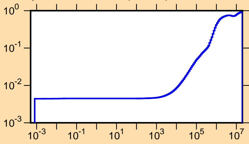
\mu vs. E for ^{153}\text{Tm}(\text{mt251})
