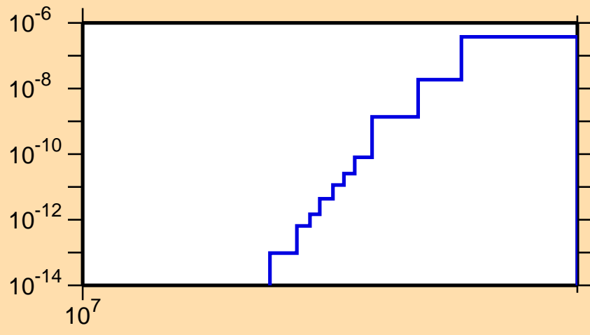
\sigma vs. E for ^{153}\text{Tm}(n,pt)
