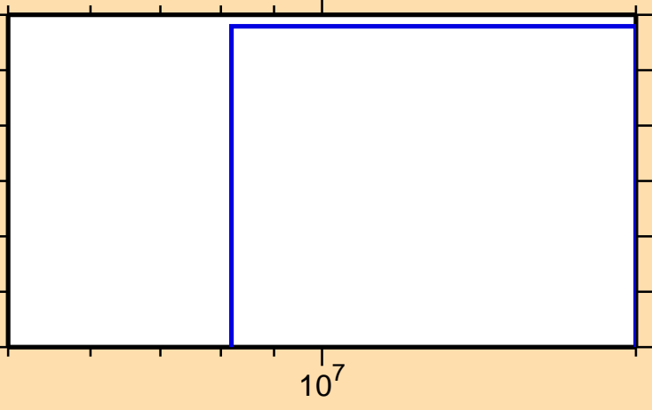
\sigma vs. E for ^{153}\text{Tm}(n,2n\alpha)
