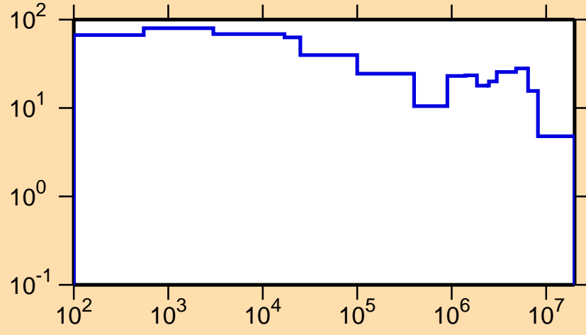
\Delta\sigma/\sigma vs. E for ^{153}\text{Tm}(n,el.)
