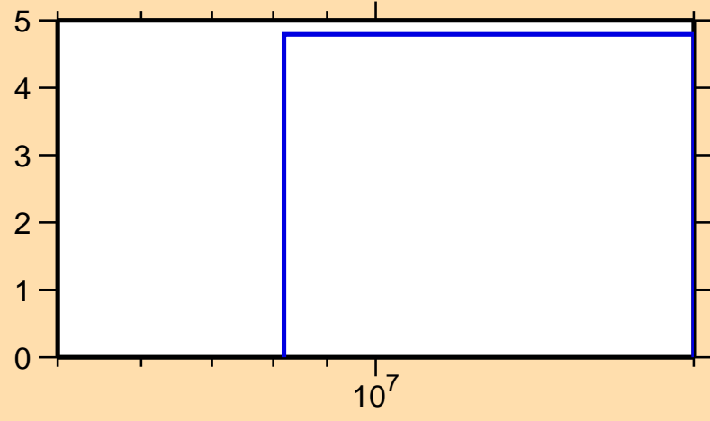
\Delta\sigma/\sigma vs. E for ^{153}\text{Tm}(n,\text{el.})
