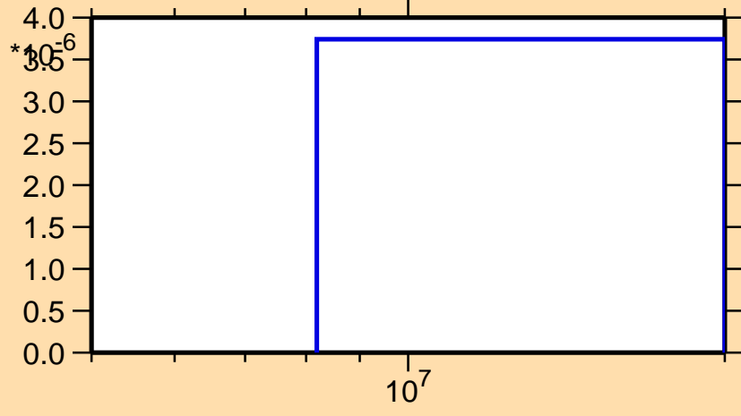
\sigma vs. E for ^{153}\text{Tm}(n,\text{pd})
