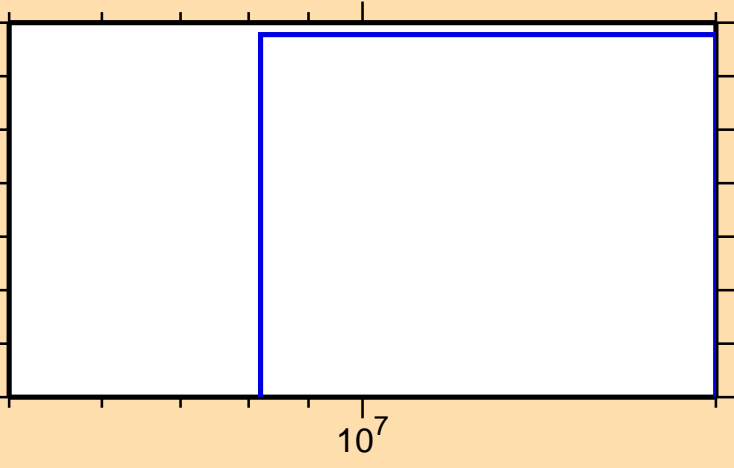
\sigma vs. E for ^{153}\text{Tm}(n,3n)
