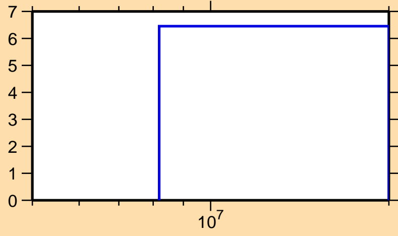
\Delta\sigma/\sigma vs. E for ^{153}\text{Tm}(n,\text{nonel.})
