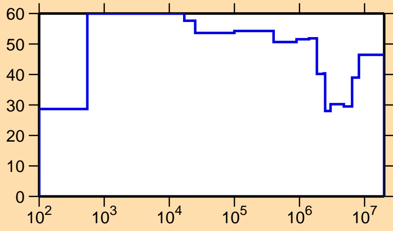
\Delta\sigma/\sigma vs. E for ^{153}\text{Tm}(n,p)
