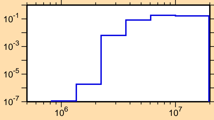
\sigma vs. E for ^{153}\text{Tm}(n,n\alpha)
