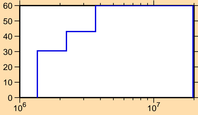
\Delta\sigma/\sigma vs. E for ^{153}\text{Tm}(n, el.)
