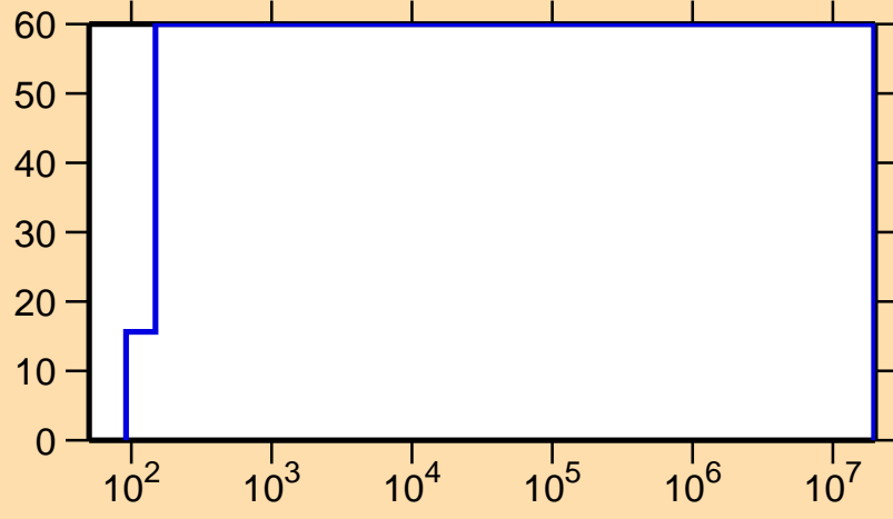
\Delta\sigma/\sigma vs. E for ^{153}\text{Tm}(n,p)
