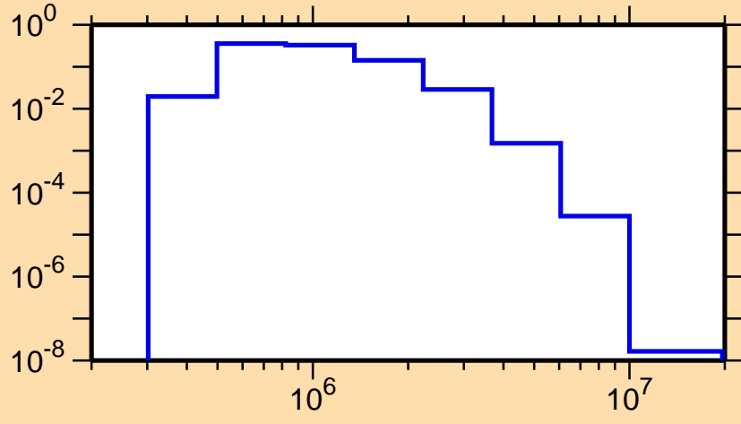
\sigma vs. E for ^{153}\text{Tm}(n,n_3)
