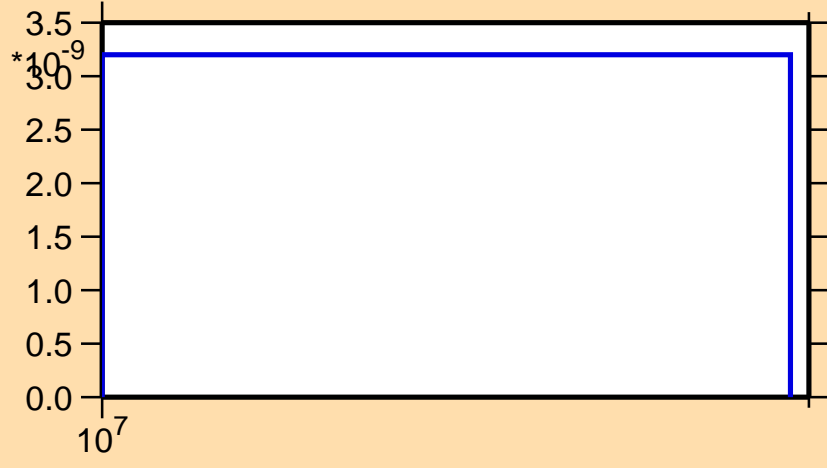
\sigma vs. E for ^{153}\text{Tm}(n,3n)
