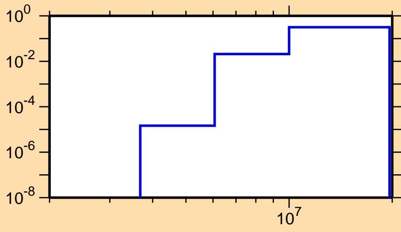
\sigma vs. E for ^{153}\text{Tm} (mt 45)
