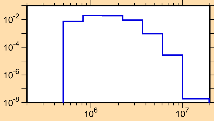
\sigma vs. E for ^{153}\text{Tm}(n,n_4)
