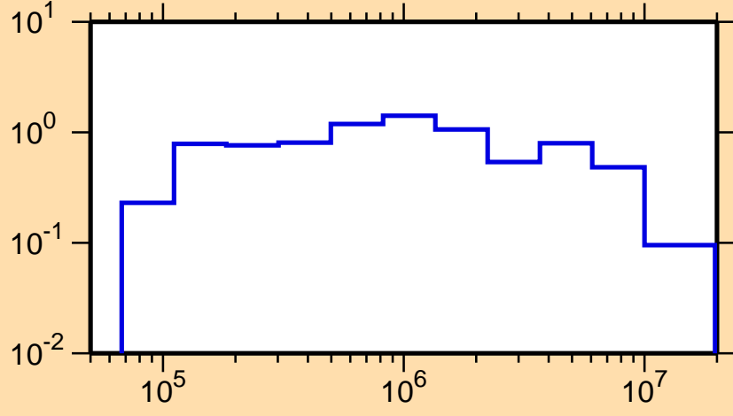
\sigma vs. E for ^{153}\text{Tm}(n,\text{inel.})
