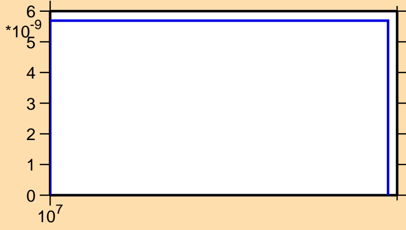
\sigma vs. E for ^{153}\text{Tm}(n,nt)
