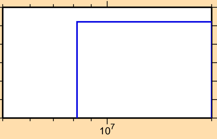
\sigma vs. E for ^{153}\text{Tm}(n,nt)
