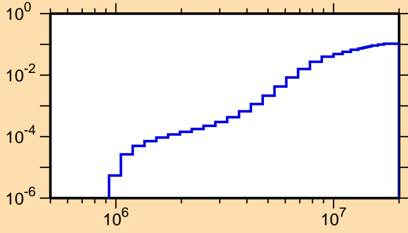
\sigma vs. E for ^{154}\text{Tm}(n,n\alpha)
