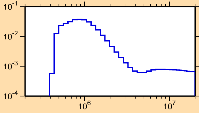
\sigma vs. E for ^{154}\text{Tm}(n,n_3)
