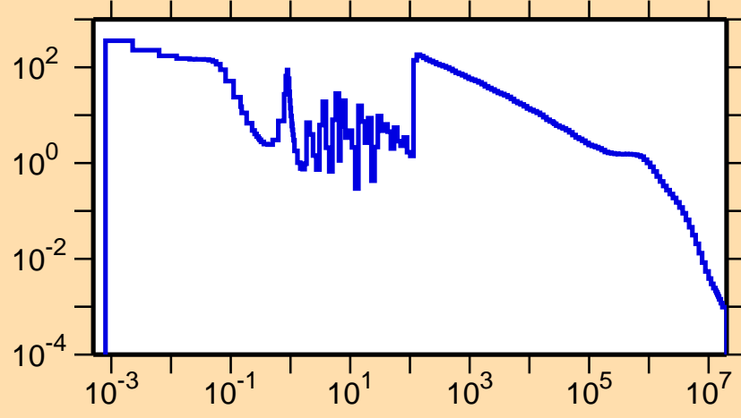
\sigma vs. E for ^{154}\text{Tm}(n,\gamma)
