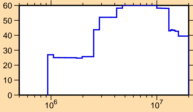
\Delta\sigma/\sigma vs. E for ^{154}\text{Tm}(n, el.)
