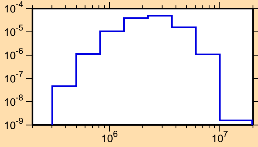
\sigma vs. E for ^{154}\text{Tm}(n,n_2)
