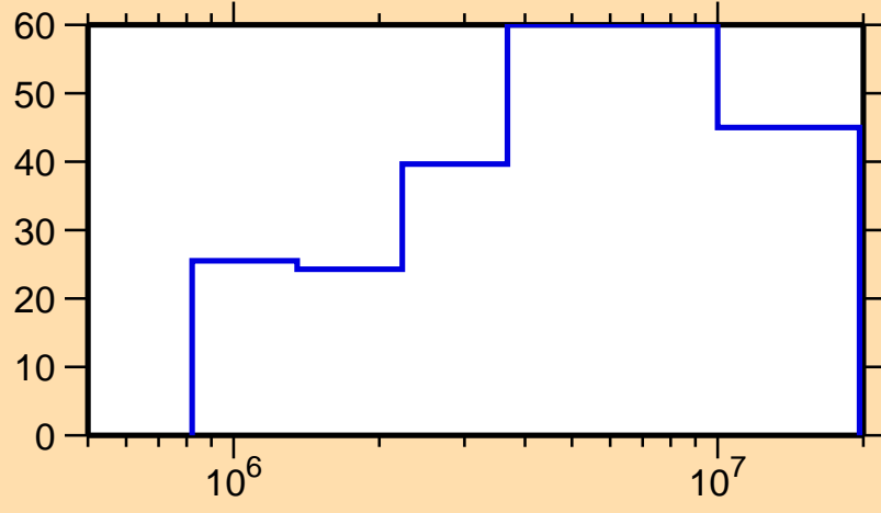
\Delta\sigma/\sigma vs. E for ^{154}\text{Tm}(n, el.)
