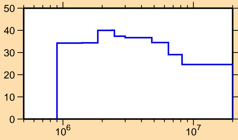
\Delta\sigma/\sigma vs. E for ^{154}\text{Tm}(n, nonel.)
