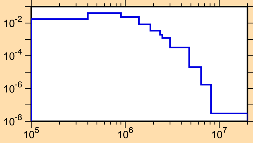
\sigma vs. E for ^{154}\text{Tm}(n,n_1)
