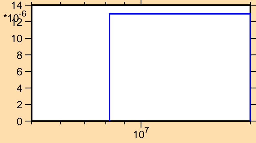
\sigma vs. E for ^{154}\text{Tm}(n,\text{nd})
