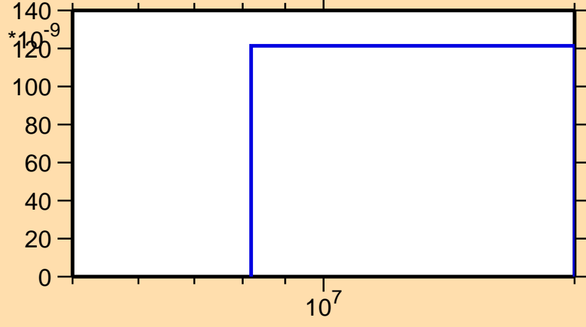
\sigma vs. E for ^{154}\text{Tm}(n,\text{pt})
