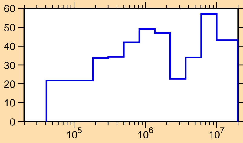
\Delta\sigma/\sigma vs. E for ^{155}\text{Tm}(n,n_1)
