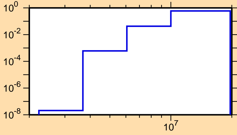
\sigma vs. E for ^{155}\text{Tm}(n,np)
