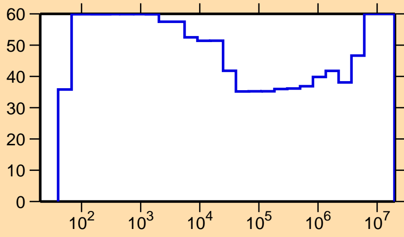
\Delta\sigma/\sigma vs. E for ^{155}\text{Tm}(n,\gamma)
