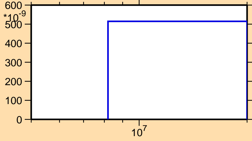
\sigma vs. E for ^{155}\text{Tm}(n,\text{nd})
