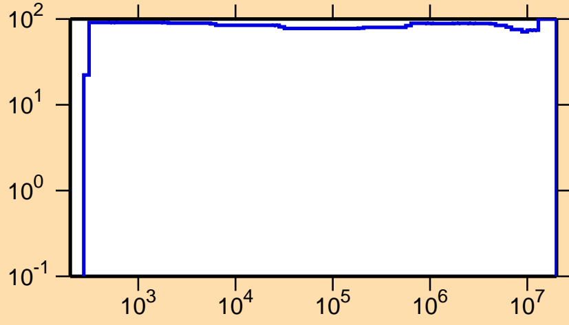
\Delta\sigma/\sigma vs. E for ^{155}\text{Tm}(n,\gamma)
