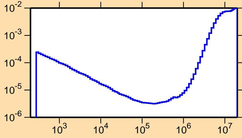
\sigma vs. E for ^{155}\text{Tm}(n,p\alpha)
