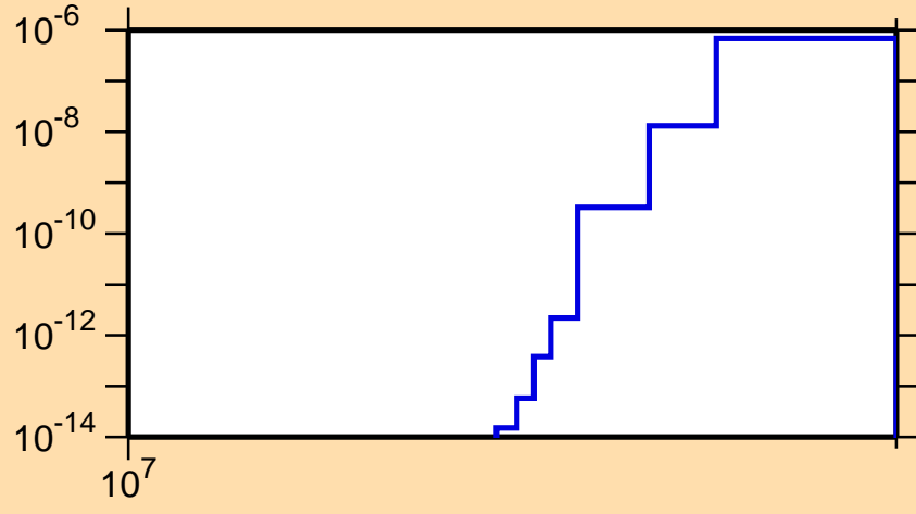
\sigma vs. E for ^{155}\text{Tm}(n,nt)
