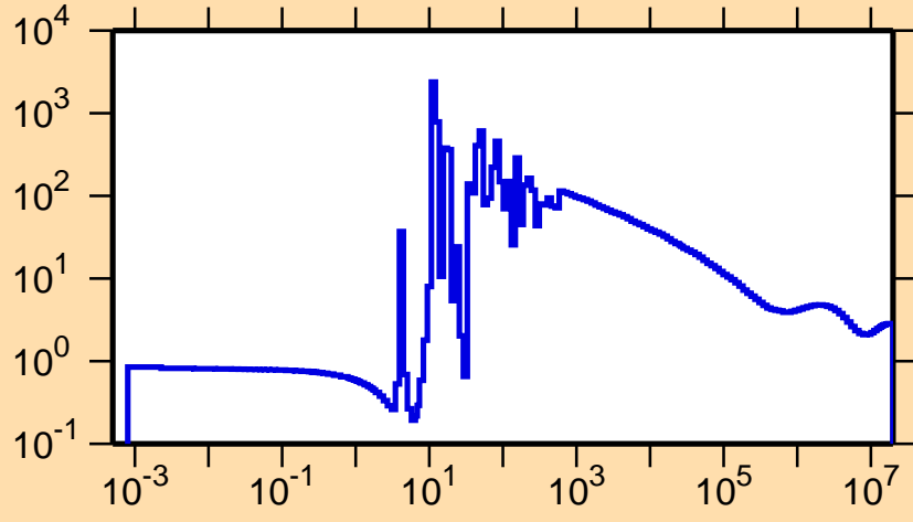
\sigma vs. E for ^{155}\text{Tm}(n,\text{el.})
