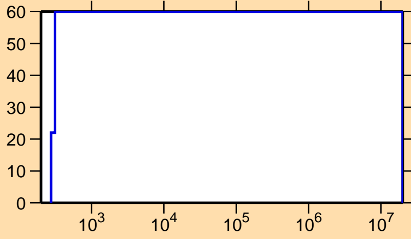
\Delta\sigma/\sigma vs. E for ^{155}\text{Tm}(n,p)
