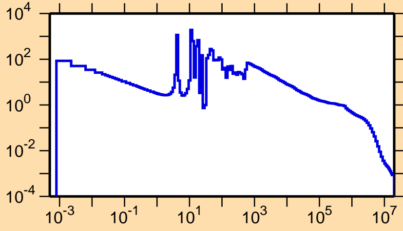
\sigma vs. E for ^{155}\text{Tm}(n,\gamma)
