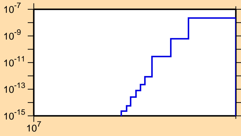
\sigma vs. E for ^{155}\text{Tm}(n,pt)
