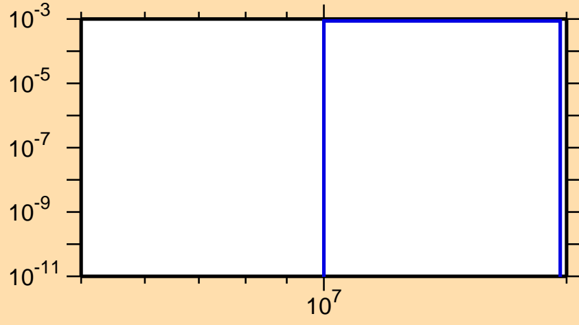
\sigma vs. E for ^{155}\text{Tm}(n,2n\alpha)
