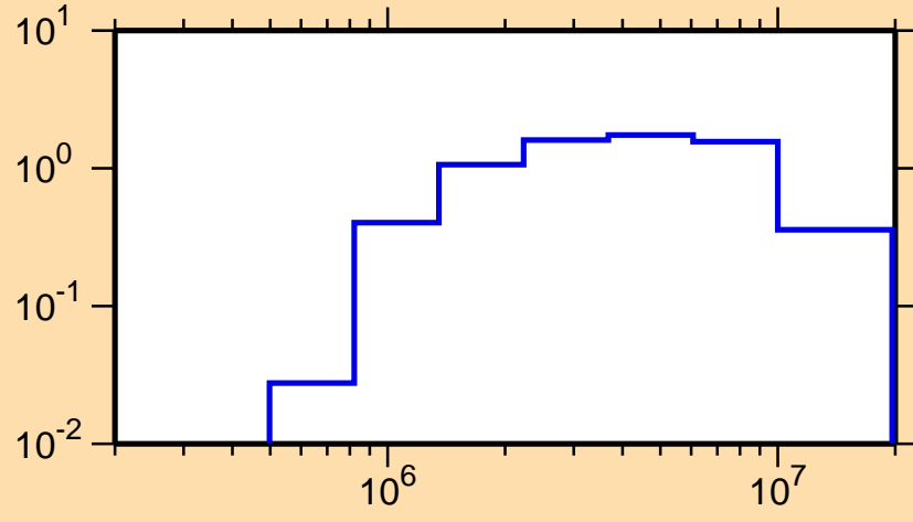
\sigma vs. E for ^{155}\text{Tm}(n,n\text{cont.})
