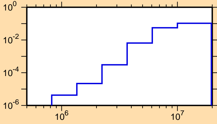
\sigma vs. E for ^{155}\text{Tm}(n,n\alpha)
