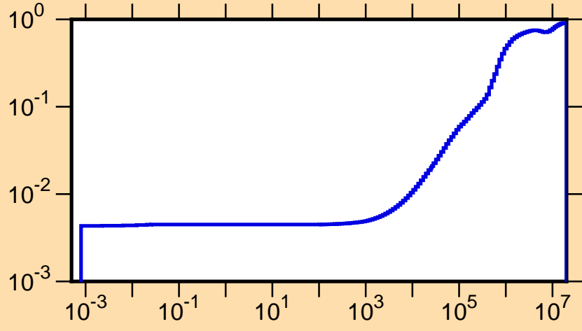
\mu vs. E for ^{156}\text{Tm}(\text{mt251})
