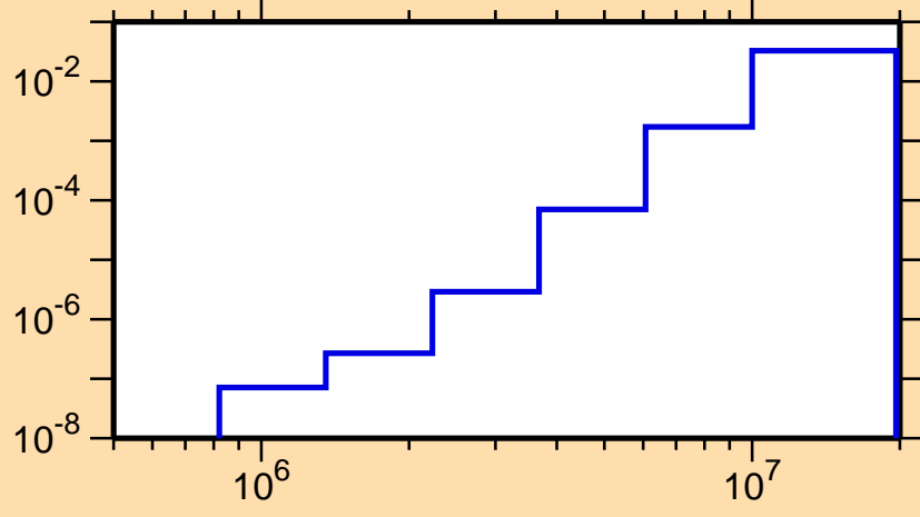
\sigma vs. E for ^{156}\text{Tm}(n,n\alpha)
