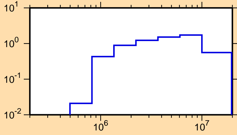
\sigma vs. E for ^{156}\text{Tm}(n,n\text{cont.})
