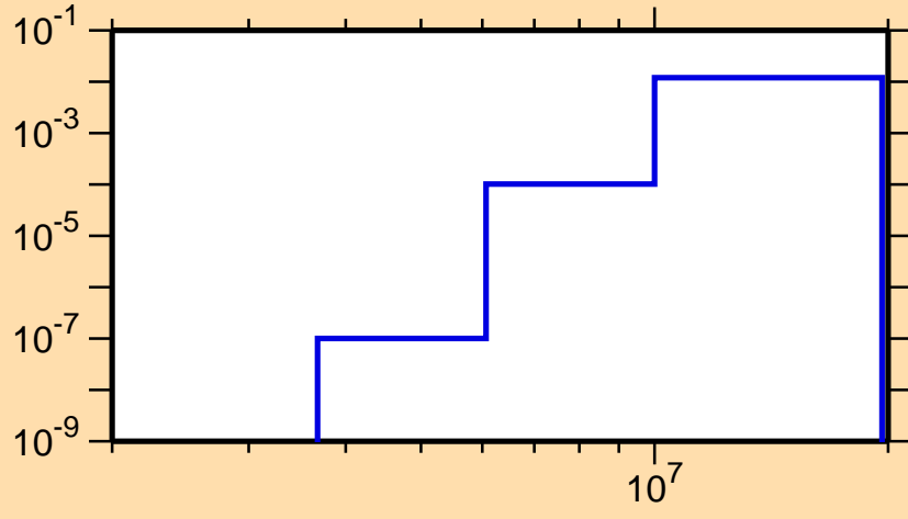
\sigma vs. E for ^{156}\text{Tm}(n,d)
