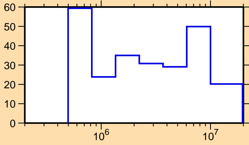
\Delta\sigma/\sigma vs. E for ^{156}\text{Tm}(n,el.)
