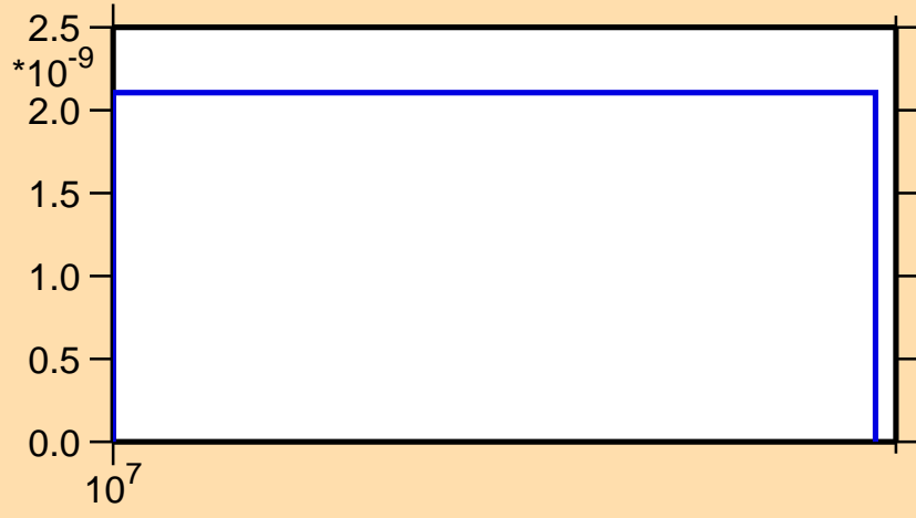
\sigma vs. E for ^{156}\text{Tm}(n,pt)
