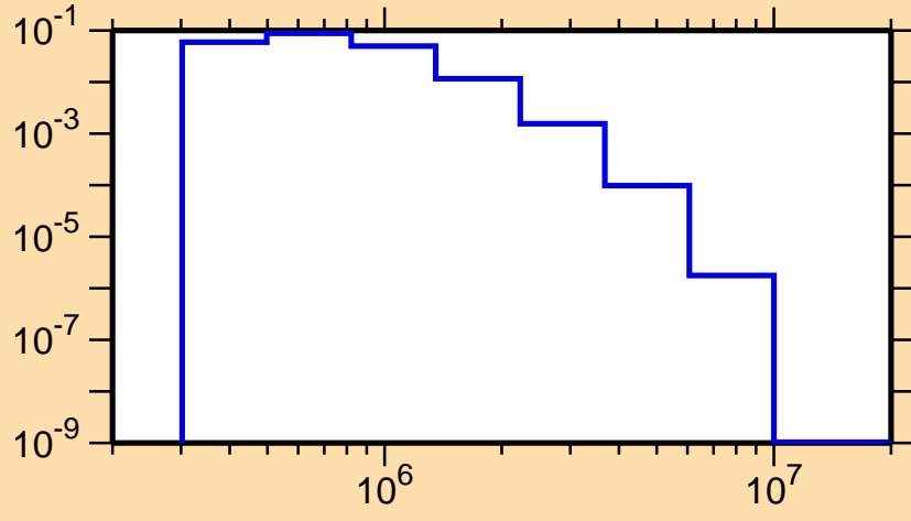
\sigma vs. E for ^{156}\text{Tm}(n,n_3)
