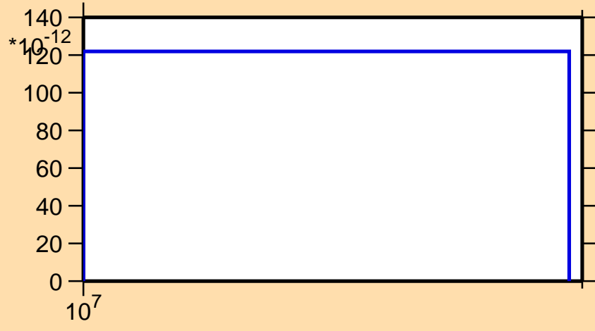
\sigma vs. E for ^{156}\text{Tm} (mt 34)
