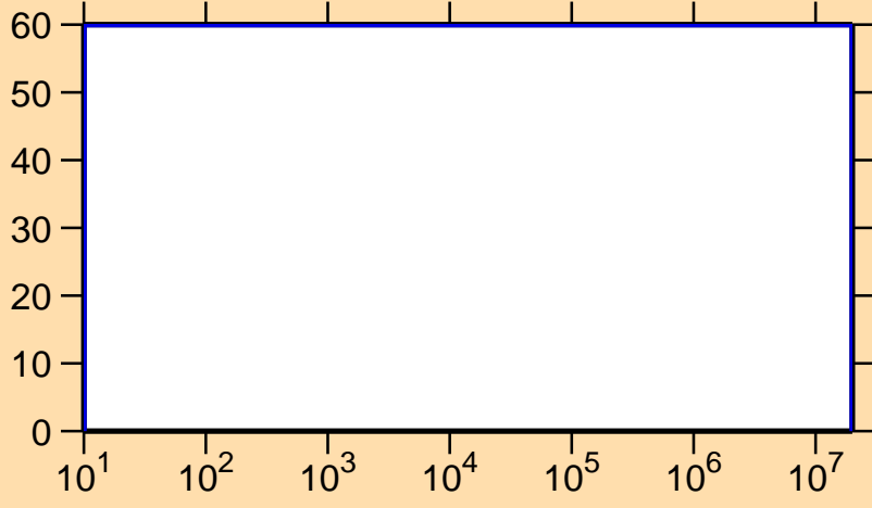
\Delta\sigma/\sigma vs. E for ^{156}\text{Tm}(n,\gamma)
