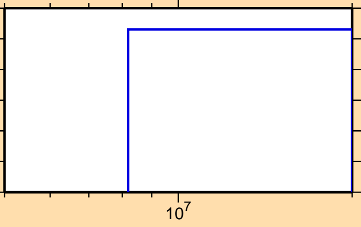
\sigma vs. E for ^{156}\text{Tm}(n,nt)
