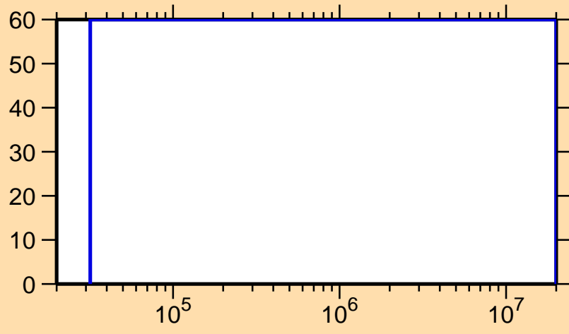
\Delta\sigma/\sigma vs. E for ^{157}\text{Tm}(n,n_1)
