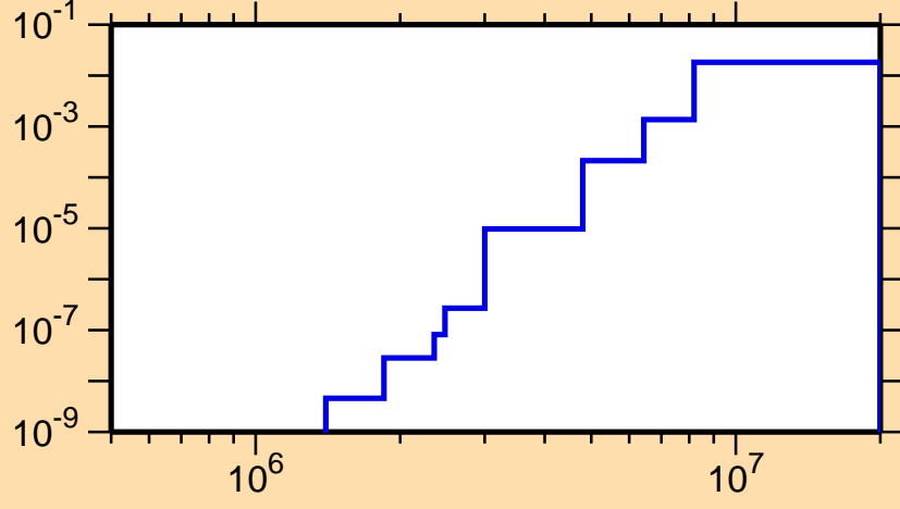
\sigma vs. E for ^{157}\text{Tm}(n,n\alpha)
