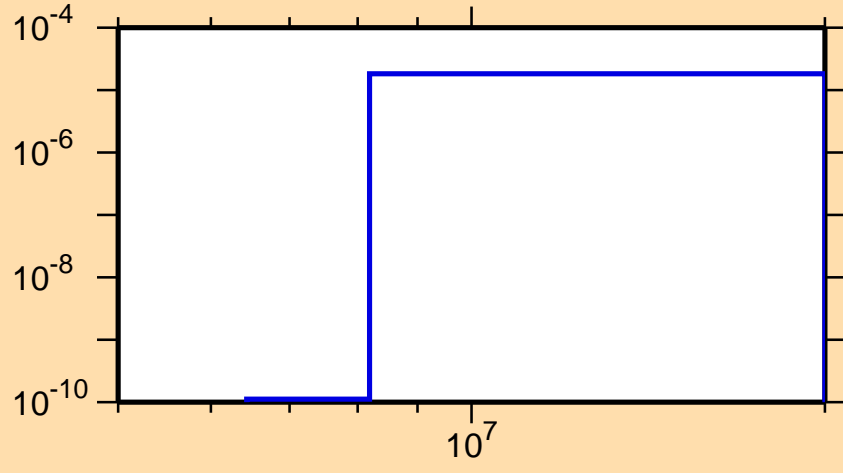
\sigma vs. E for ^{157}\text{Tm} (mt 45)
