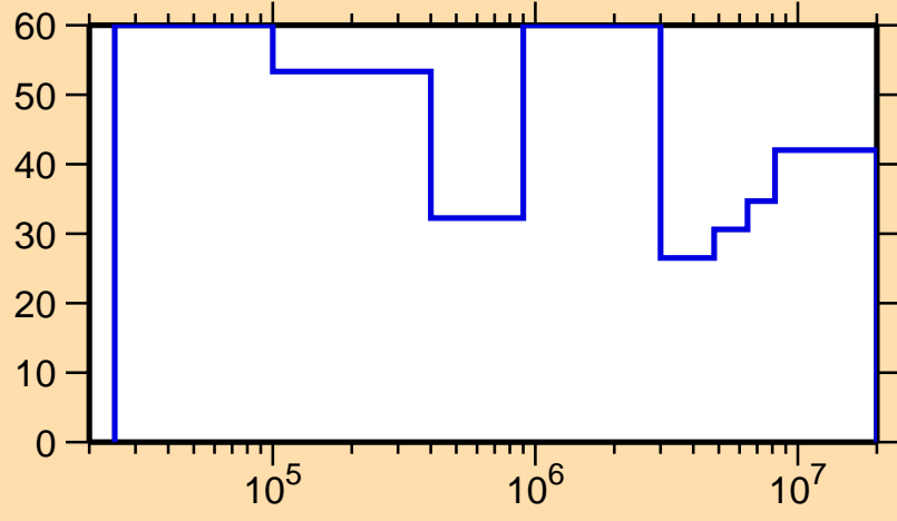
\Delta\sigma/\sigma vs. E for ^{157}\text{Tm}(n,\text{inel.})
