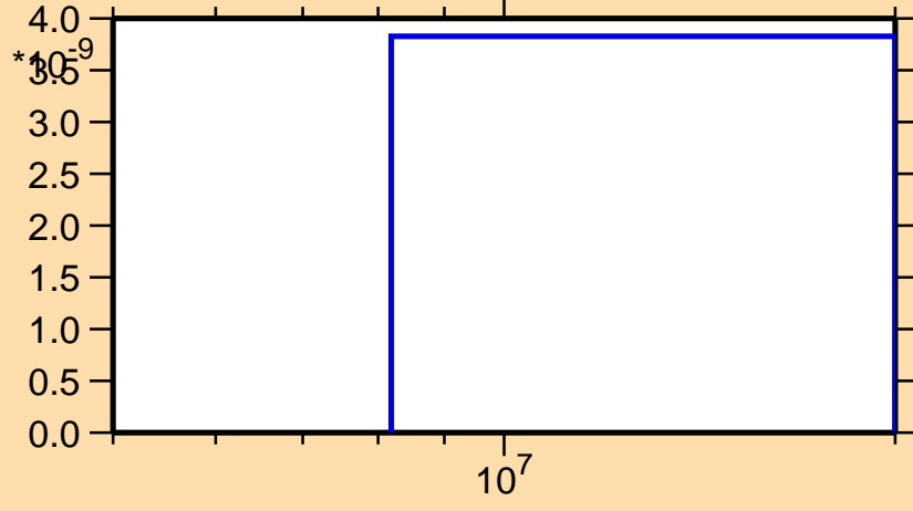
\sigma vs. E for ^{157}\text{Tm}(n,nt)
