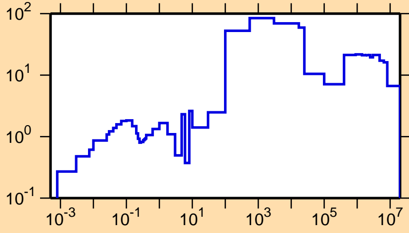
\Delta\sigma/\sigma vs. E for ^{157}\text{Tm}(n,\text{tot.})
