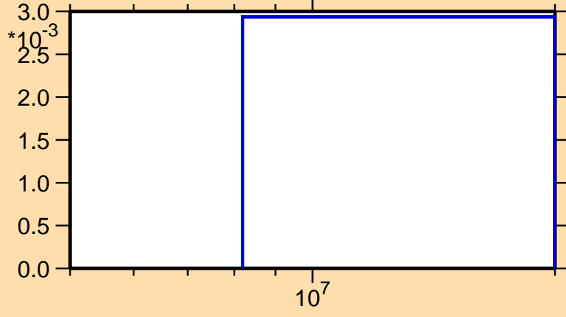
\sigma vs. E for ^{157}\text{Tm}(n,2n\alpha)
