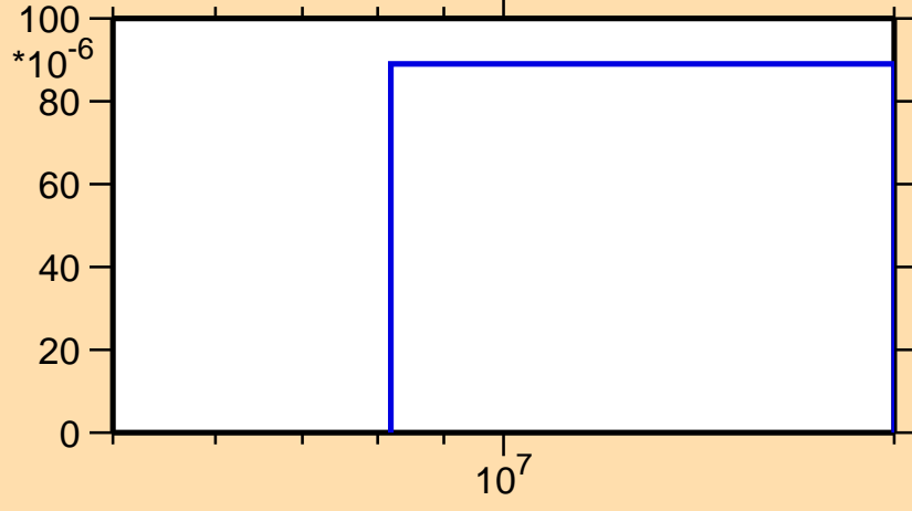
\sigma vs. E for ^{157}\text{Tm}(n,2np)
