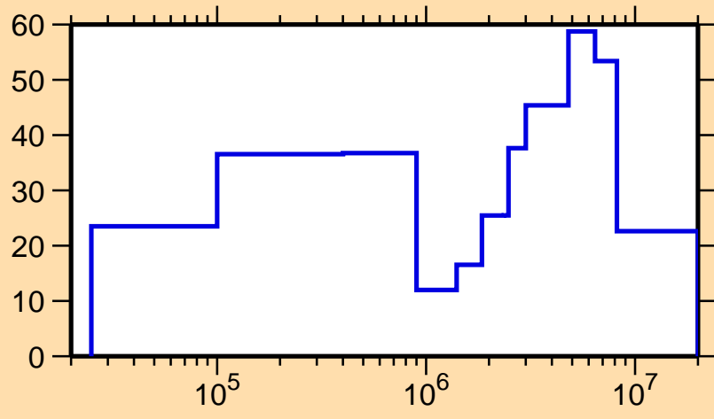
\Delta\sigma/\sigma vs. E for ^{157}\text{Tm}(n,\text{el.})
