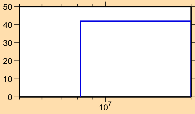
\Delta\sigma/\sigma vs. E for ^{157}\text{Tm}(n,\text{inel.})
