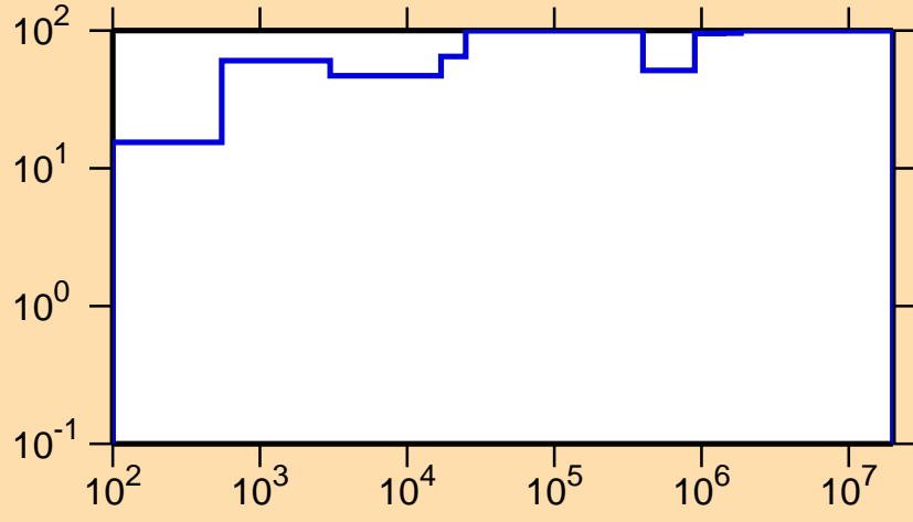
\Delta\sigma/\sigma vs. E for ^{157}\text{Tm}(n,p)
