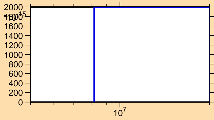
\sigma vs. E for ^{157}\text{Tm}(n,\text{pt})
