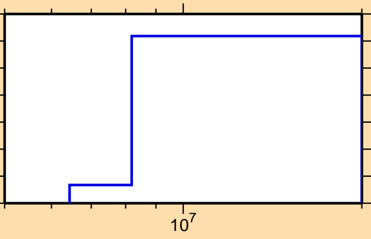
\sigma vs. E for ^{157}\text{Tm}(\text{mt117})
