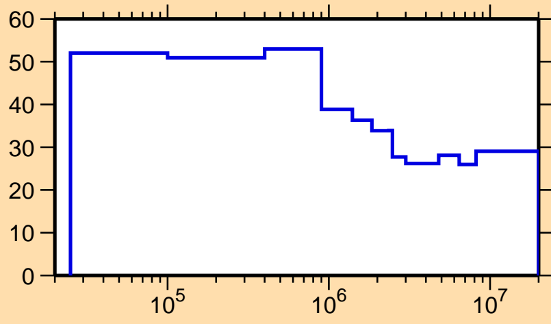
\Delta\sigma/\sigma vs. E for ^{157}\text{Tm}(n,\text{nonel.})
