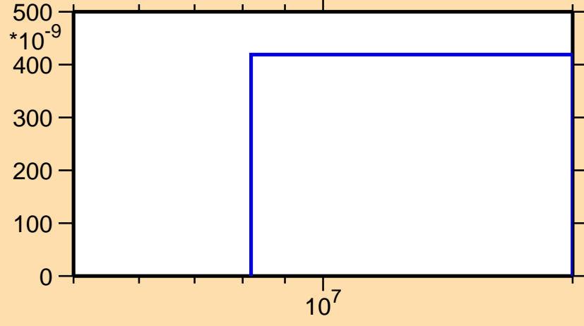
\sigma vs. E for ^{157}\text{Tm}(n,nd)
