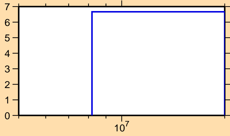
\Delta\sigma/\sigma vs. E for ^{157}\text{Tm}(n,\text{tot.})
