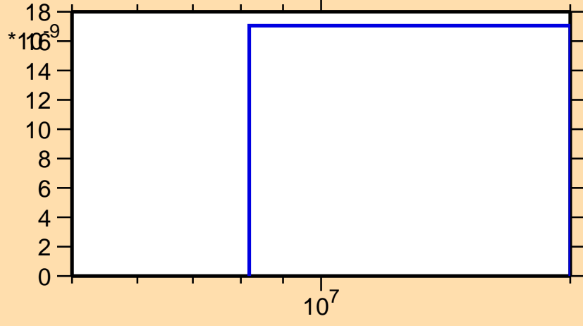
\sigma vs. E for ^{157}\text{Tm}(n,3n\alpha)
