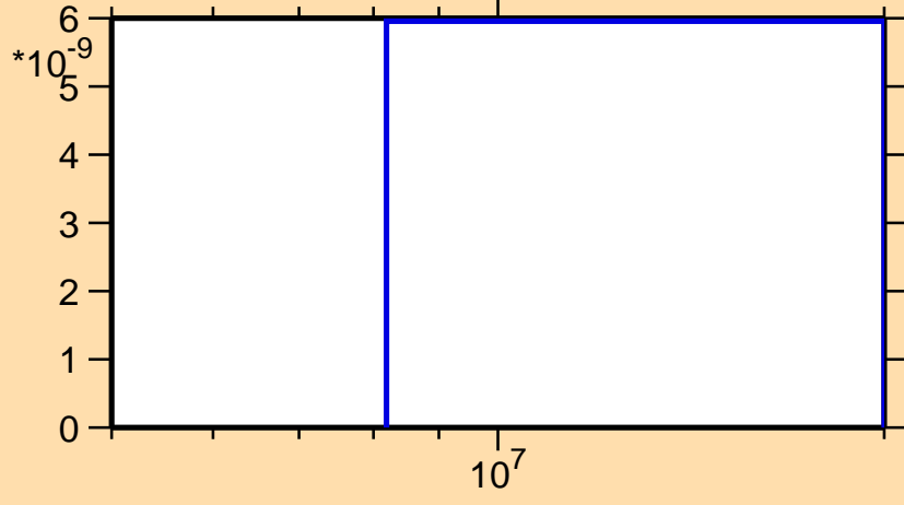
\sigma vs. E for ^{157}\text{Tm}(n,\text{pd})
