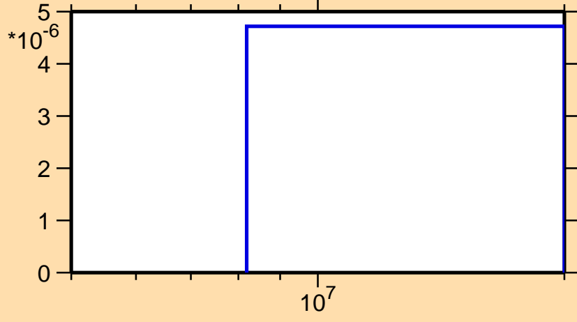
\sigma vs. E for ^{157}\text{Tm}(n,3n)
