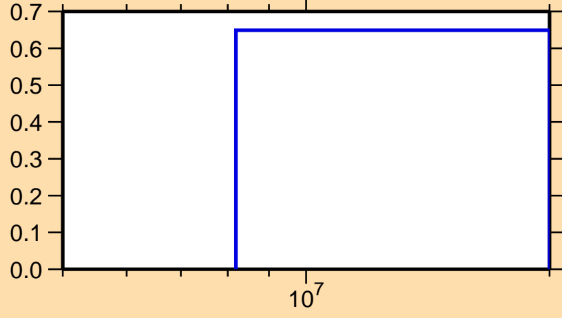
\sigma vs. E for ^{157}\text{Tm}(n,2n)
