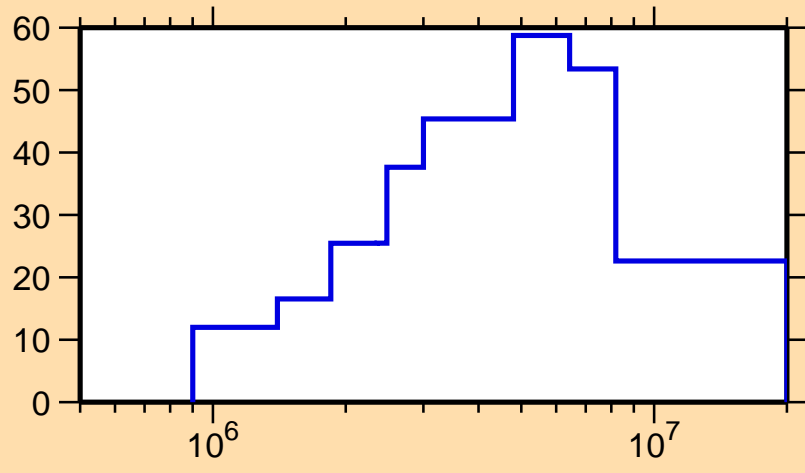
\Delta\sigma/\sigma vs. E for ^{157}\text{Tm}(n, el.)
