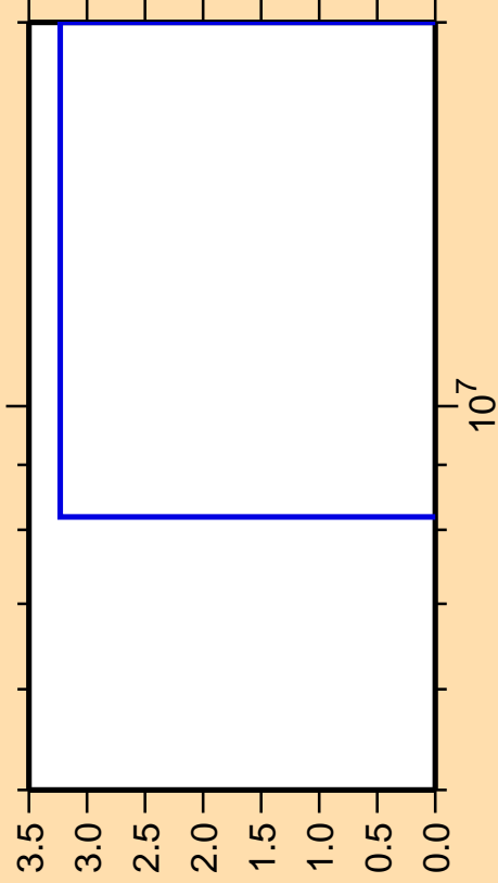
\Delta\sigma/\sigma vs. E for ^{157}\text{Tm} (mt 34)
