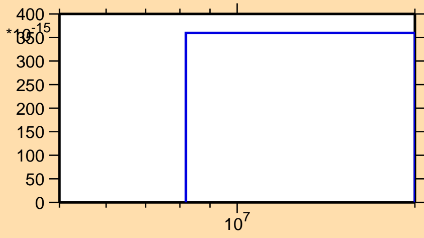
\sigma vs. E for ^{157}\text{Tm} (mt 34)
