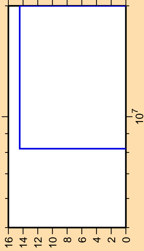
\Delta\sigma/\sigma vs. E for ^{157}\text{Tm}(n,\text{pt})
