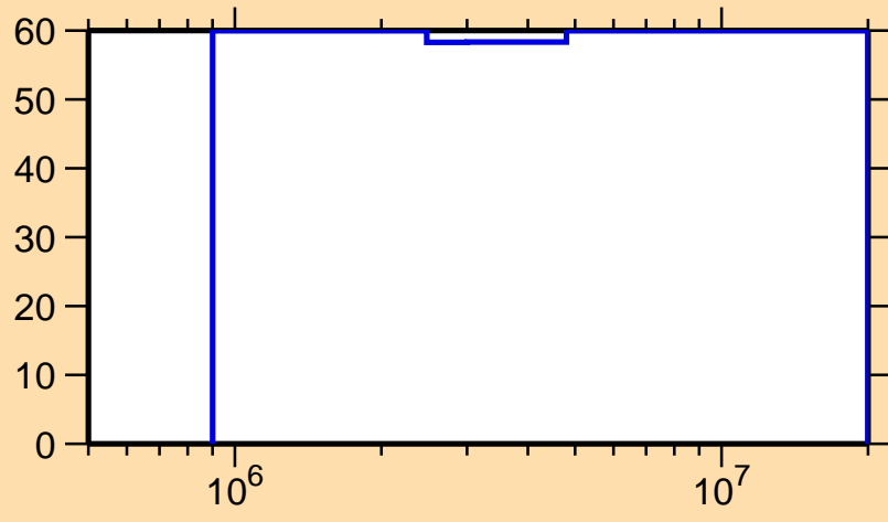
\Delta\sigma/\sigma vs. E for ^{157}\text{Tm}(n,n\text{cont.})
