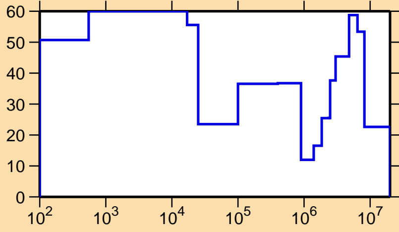
\Delta\sigma/\sigma vs. E for ^{157}\text{Tm}(n,\text{el.})
