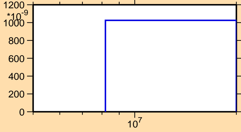
\sigma vs. E for ^{157}\text{Tm}(n,\text{He}3)
