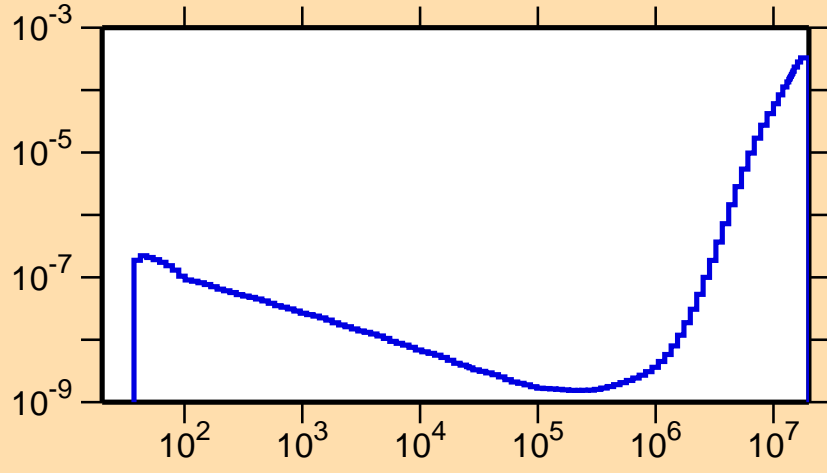
\sigma vs. E for ^{158}\text{Tm}(n,p\alpha)
