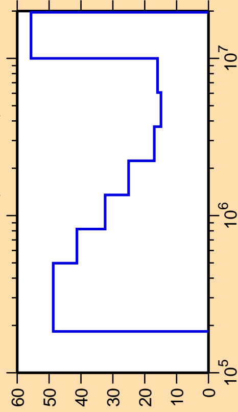
\Delta\sigma/\sigma vs. E for ^{158}\text{Tm}(n,ncont.)
