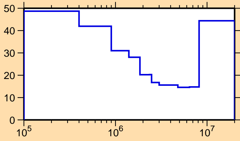
\Delta\sigma/\sigma vs. E for ^{158}\text{Tm}(n,ncont.)
