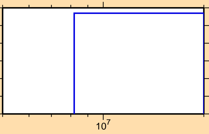
\sigma vs. E for ^{158}\text{Tm}(n,nt)
