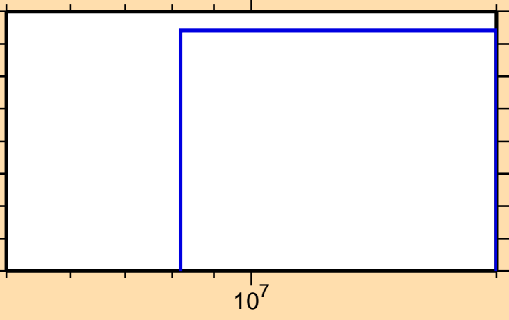
\sigma vs. E for ^{158}\text{Tm}(n,\text{nd})
