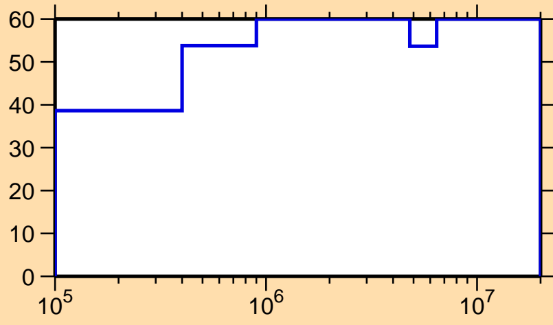
\Delta\sigma/\sigma vs. E for ^{158}\text{Tm}(n,n_1)
