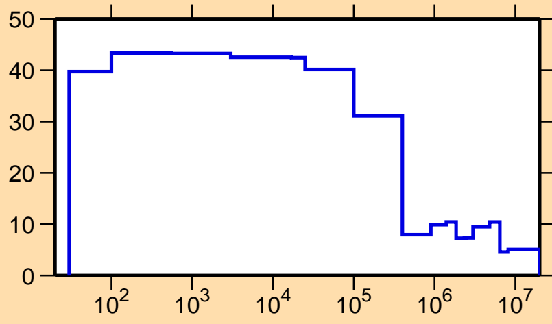
\Delta\sigma/\sigma vs. E for ^{158}\text{Tm}(n,el.)
