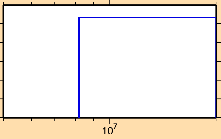
\sigma vs. E for ^{158}\text{Tm}(\text{mt117})
