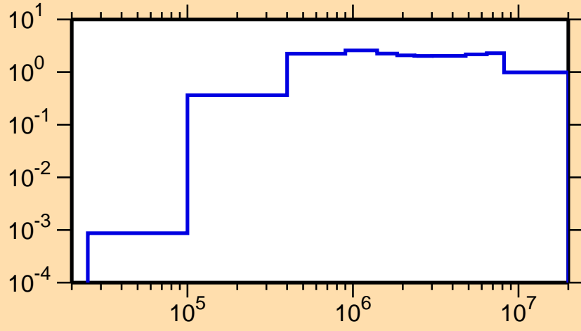
\sigma vs. E for ^{158}\text{Tm}(n,\text{inel.})
