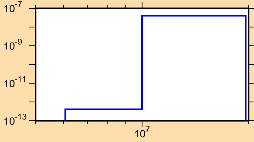
\sigma vs. E for ^{158}\text{Tm}(\text{mt117})
