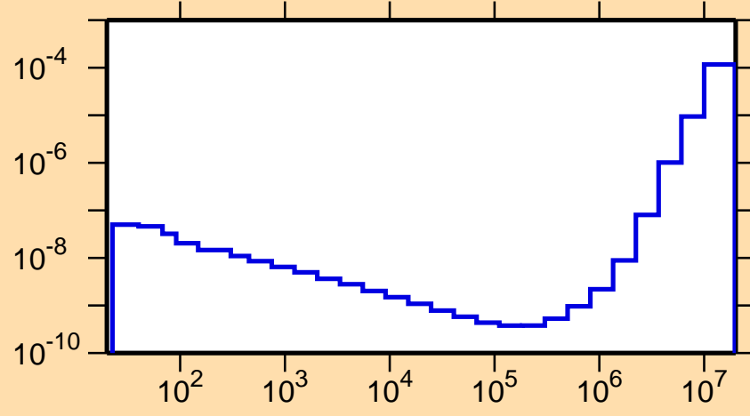
\sigma vs. E for ^{158}\text{Tm}(n,p\alpha)
