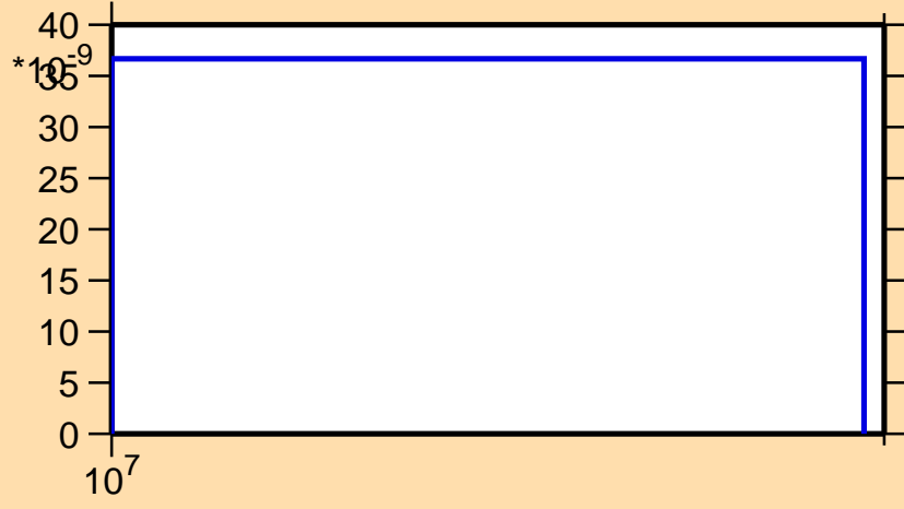
\sigma vs. E for ^{158}\text{Tm}(n,3n\alpha)
