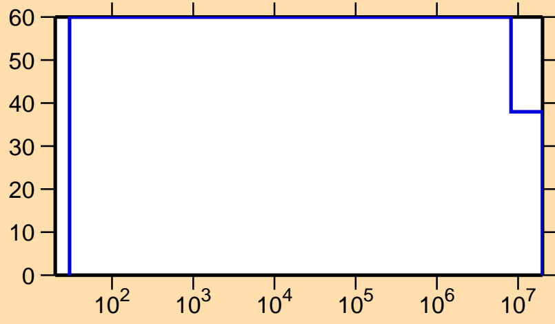
\Delta\sigma/\sigma vs. E for ^{158}\text{Tm}(n,p)
