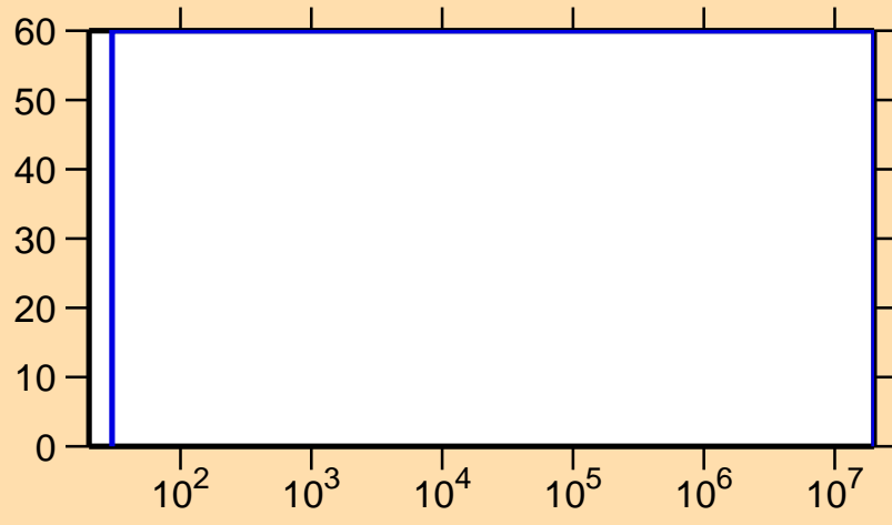
\Delta\sigma/\sigma vs. E for ^{158}\text{Tm}(n,\gamma)
