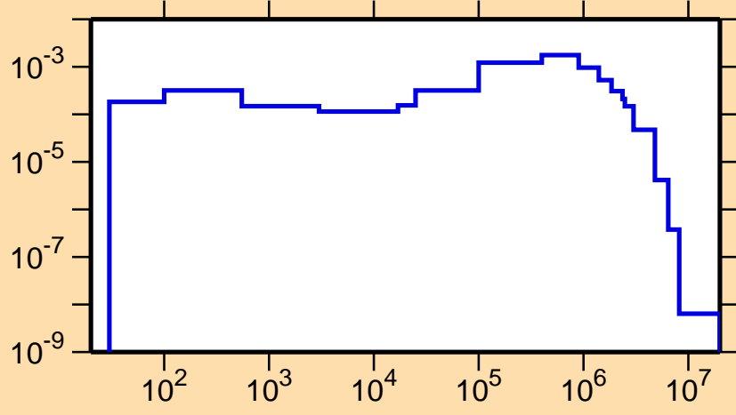
\sigma vs. E for ^{158}\text{Tm}(n,n_1)
