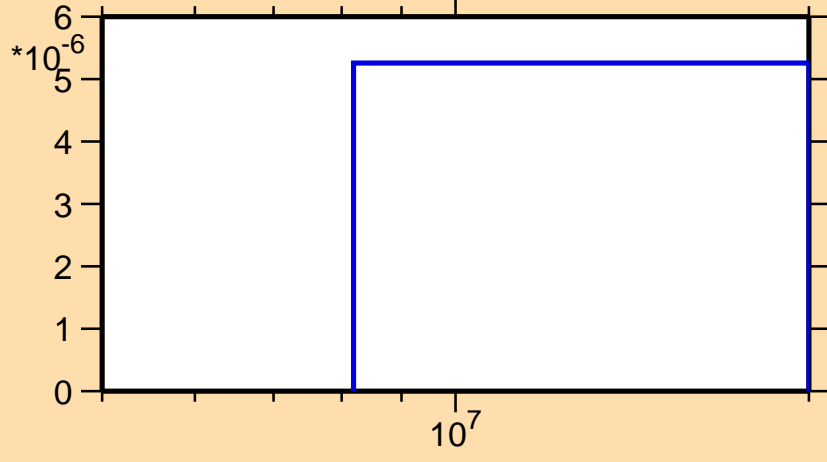
\sigma vs. E for ^{158}\text{Tm}(n,\text{nd})
