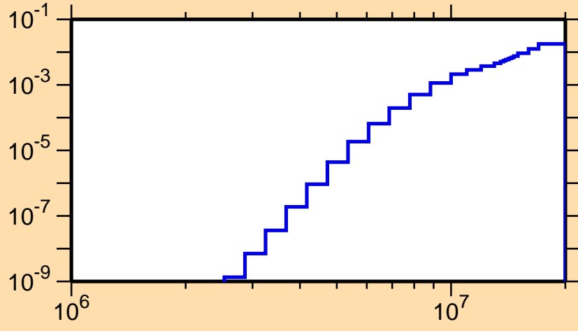
\sigma vs. E for ^{159}\text{Tm}(n,n\alpha)
