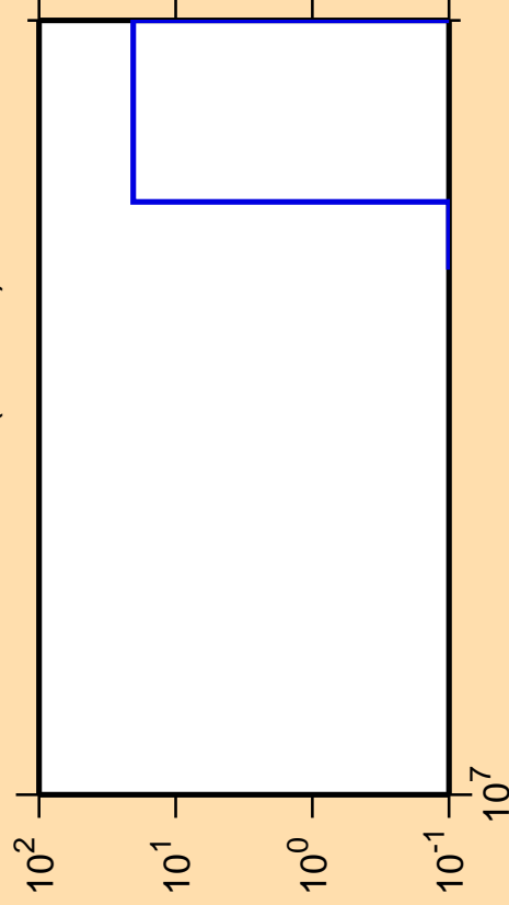
\Delta\sigma/\sigma vs. E for ^{159}\text{Tm}(n,3n\alpha)
