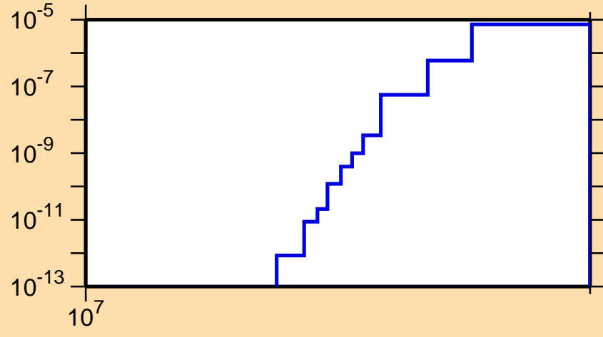
\sigma vs. E for ^{159}\text{Tm}(n,nd)
