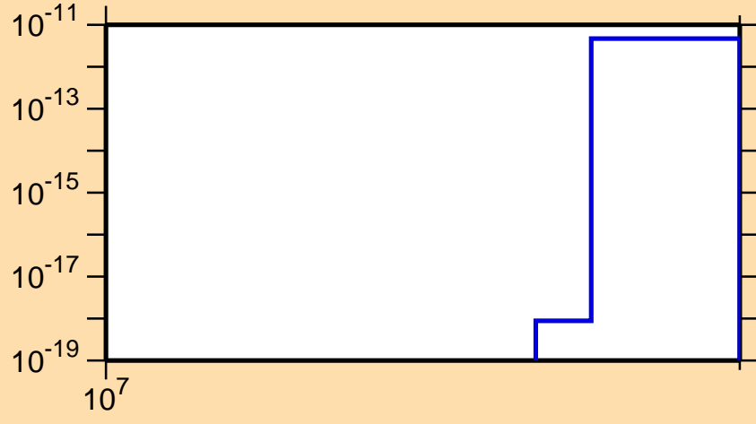
\sigma vs. E for ^{159}\text{Tm}(n,3n\alpha)
