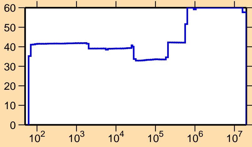
\Delta\sigma/\sigma vs. E for ^{159}\text{Tm}(n,p)
