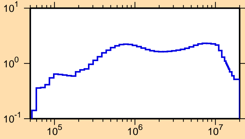
\sigma vs. E for ^{159}\text{Tm}(n,\text{inel.})
