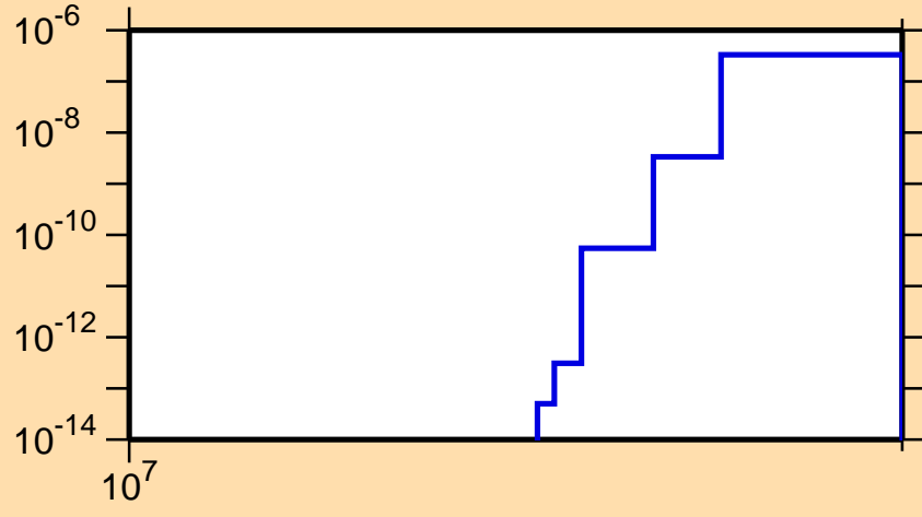
\sigma vs. E for ^{159}\text{Tm}(n,nt)
