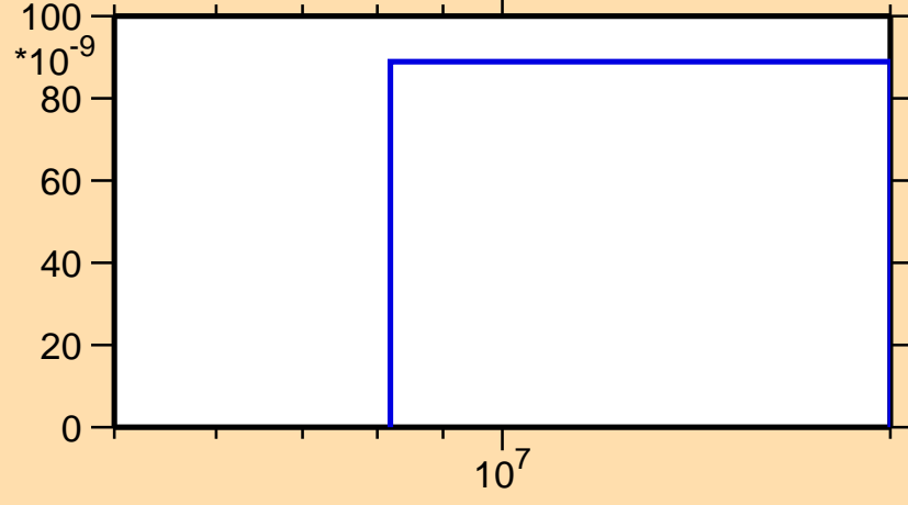
\sigma vs. E for ^{159}\text{Tm}(n,\text{nd})
