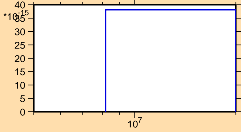
\sigma vs. E for ^{159}\text{Tm}(n,3n\alpha)
