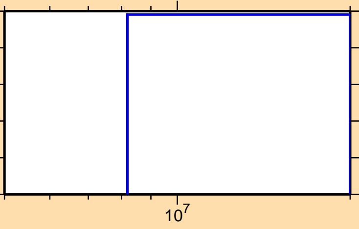
\sigma vs. E for ^{159}\text{Tm}(\text{mt117})
