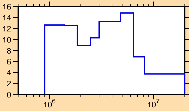
\Delta\sigma/\sigma vs. E for ^{159}\text{Tm}(n, el.)
