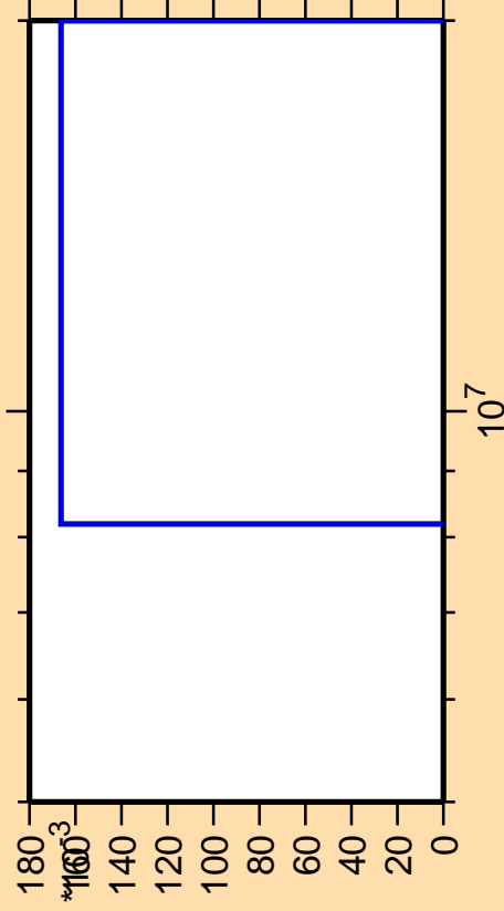
\Delta\sigma/\sigma vs. E for ^{159}\text{Tm}(n,3n\alpha)
