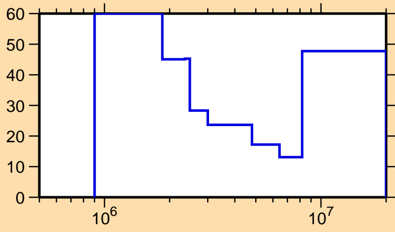
\Delta\sigma/\sigma vs. E for ^{159}\text{Tm}(n,n\text{cont.})
