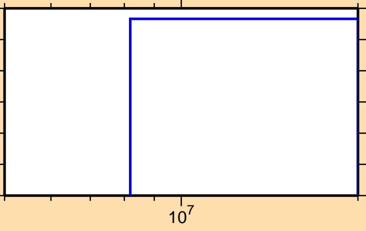
\sigma vs. E for ^{159}\text{Tm}(n,nt)
