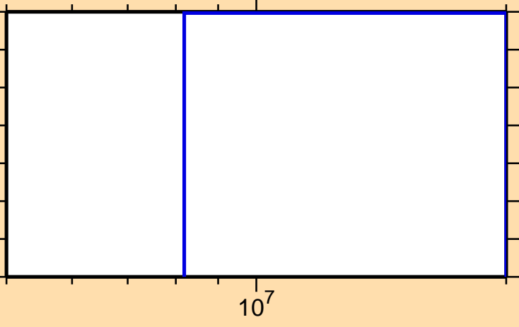
\sigma vs. E for ^{159}\text{Tm}(n,3n)
