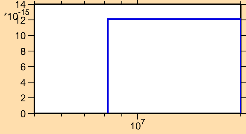
\sigma vs. E for ^{159}\text{Tm}(n,\text{pt})
