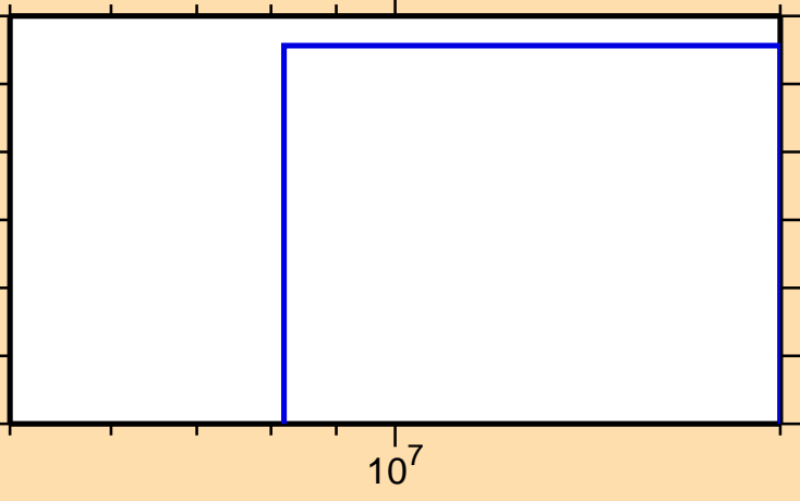
\sigma vs. E for ^{159}\text{Tm}(n,\text{pd})
