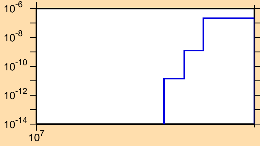
\sigma vs. E for ^{160}\text{Tm}(n,nt)
