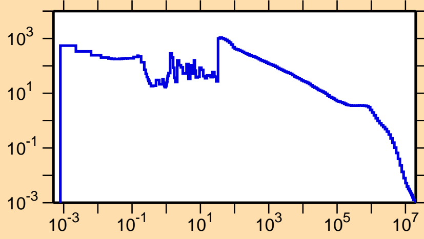
\sigma vs. E for ^{160}\text{Tm}(n,\gamma)
