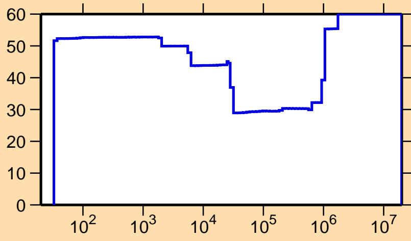
\Delta\sigma/\sigma vs. E for ^{160}\text{Tm}(n,\gamma)
