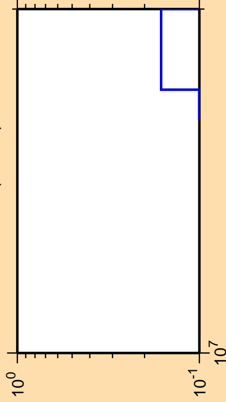
\Delta\sigma/\sigma vs. E for ^{160}\text{Tm}(n,3n\alpha)
