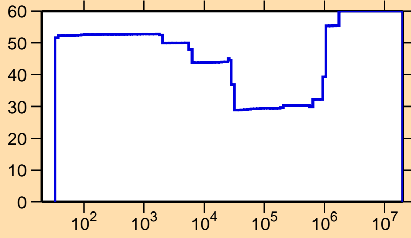
\Delta\sigma/\sigma vs. E for ^{160}\text{Tm}(n,\gamma)
