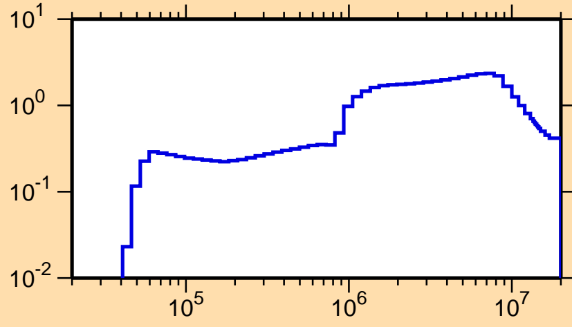
\sigma vs. E for ^{160}\text{Tm}(n,\text{inel.})
