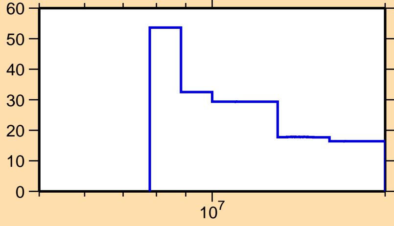
\Delta\sigma/\sigma vs. E for ^{160}\text{Tm}(n,2n)
